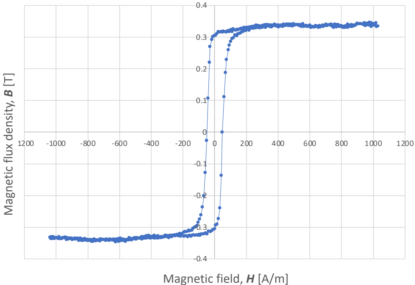
42Cu50Ni Magnetic flux density, B vs H
