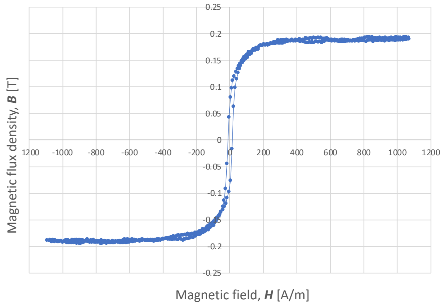
45Cu50Ni Magnetic flux density, B vs H
