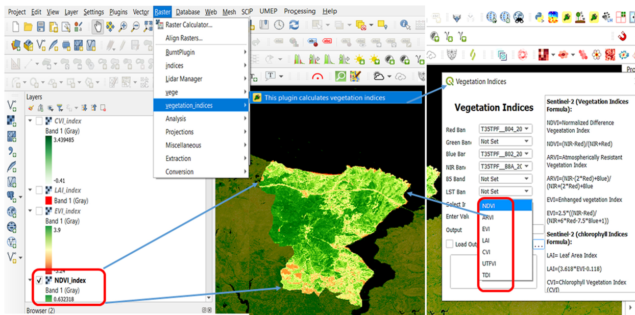
Figure 2. Overview of QSVI plugin functionalities developed by Nuray Baş. The screenshot shows the custom plugin in the QGIS interface ( https://qgis.org ).
