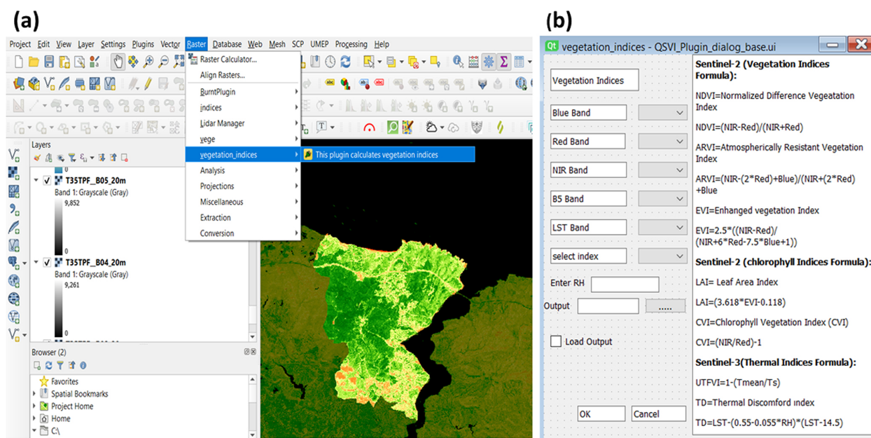
Figure 1. (a) Plugin menu tab on the QGIS platform, (b) Tabs of the QSVI graphical user interface. The screenshot is from the QGIS interface ( https://qgis.org , last access: 10 June 2025) showing the custom QSVI plugin. The plugin was developed by the author.
