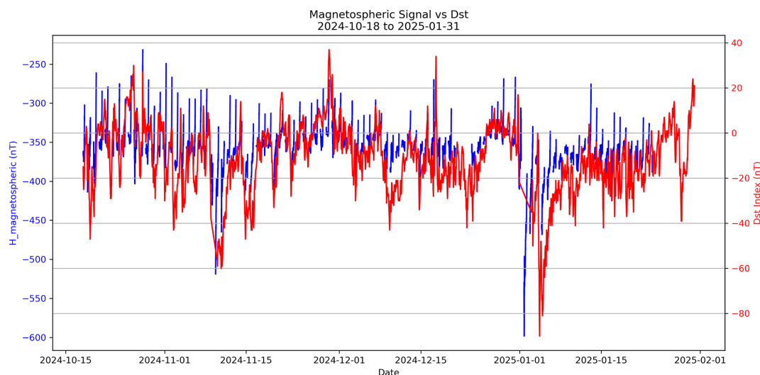
Figure 10. The measured magnetospheric signal of the station vs. the global Dst index for date range 18 October 2024–31 January 2025.
