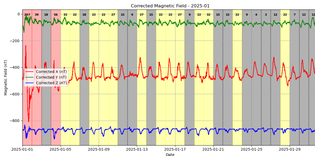
Figure 9. Variations in the local geomagnetic field along the X (red line), Y (green line), and Z (blue line) components during January 2025. As described in Fig. 5.
