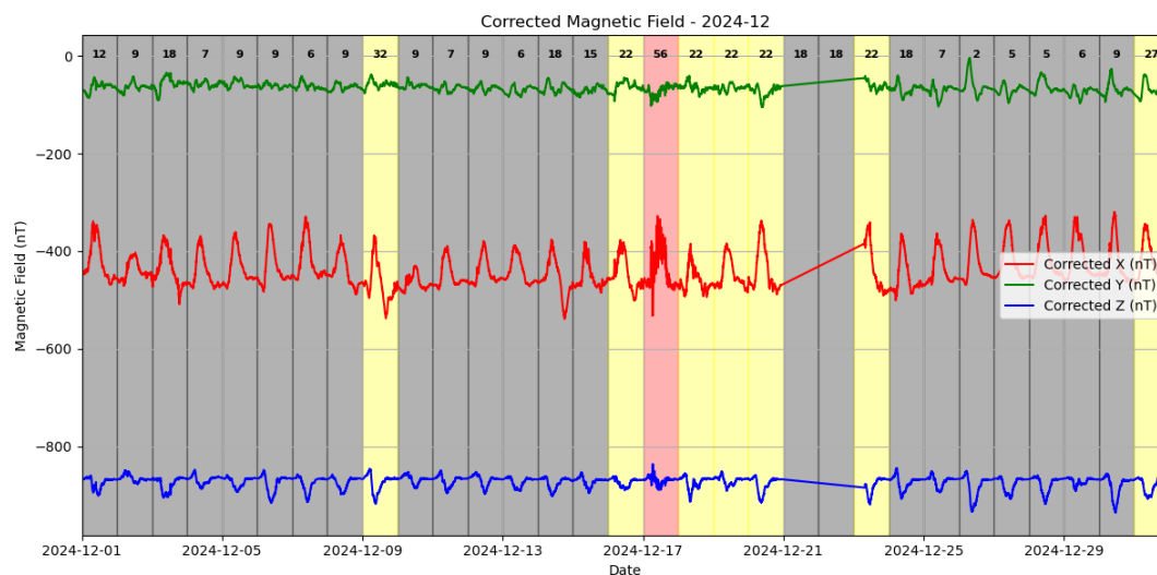
Figure 7. Variations in the local geomagnetic field along the X (red line), Y (green line), and Z (blue line) components during December 2024. As described in Fig. 5.
