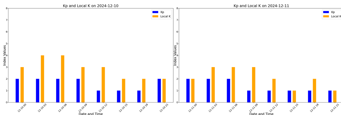
Figure 8. Kp and local K indices derived from the Entoto station. These figures show indices during quiet times, as seen in Fig. 7.
