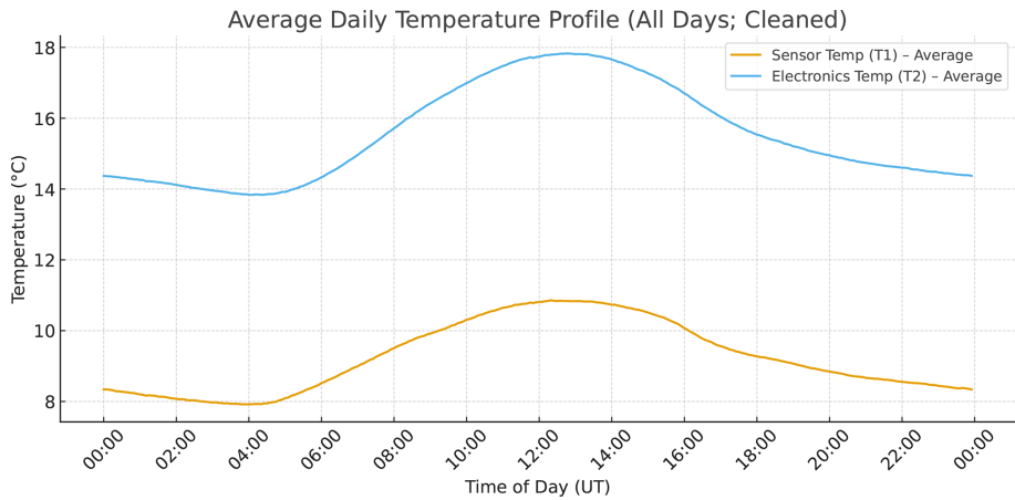
Figure 3. Average daily temperature profile inside the Entoto station enclosure, derived from all days of the last months .sec data (9 August–9 September 2025). Sensor temperature (T1) and electronics temperature (T2) both show modest diurnal variations (median daily ranges of ~ 3.5 and ~ 4.6 °C, respectively), confirming that the enclosure moderates the thermal environment.
