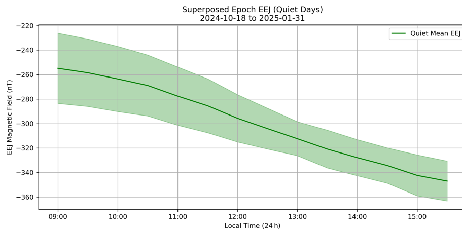
Figure 11. Mean EEJ amplitude for selected quiet geomagnetic days for the selected date range, based on the daily mean of 1 min EEJ values. These values provide a baseline for comparison with disturbed-time EEJ enhancements.
