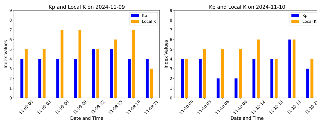
Figure 6. Kp and local K indices derived from the Entoto station. These figures show indices as measured during disturbed storm times, as seen in Fig. 5.
