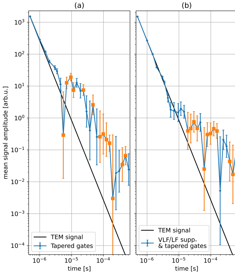
Figure 4. Sounding curve for a synthetic data example with a t^{-5/2} TEM signal, four VLF / LF radio stations, and white Gaussian noise. Left: semi-tapered gating and stacking. Right: noise suppression with VLF / LF modeling and subtraction is applied prior to semi-tapered gating and stacking. Positive signal values are plotted in blue, negative signal values are sign-changed and plotted in orange.
