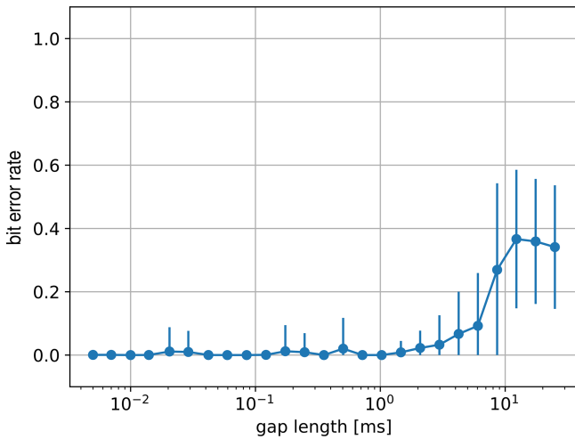
Figure 2. Bit error rate as a function of the gap length computed for a 2048 \mu\text{s} transient length. The lower part of the error bars are truncated at zero.
