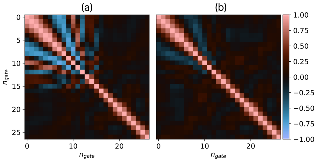
Figure 7. Covariance matrices for the noise-only field data set with an embedded artificial t^{-5/2} TEM signal.
