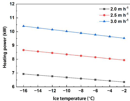
Figure 3. Calculation of power consumption.
