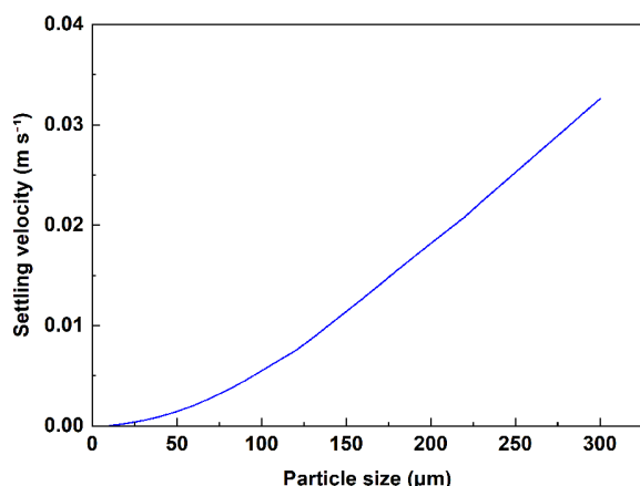
Figure 6. Effect of particle size on settling velocity.
