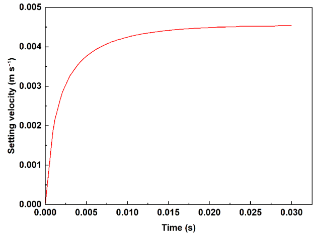
Figure 5. Temporal evolution of simulated settling velocity for 100 \mu\text{m} particles.
