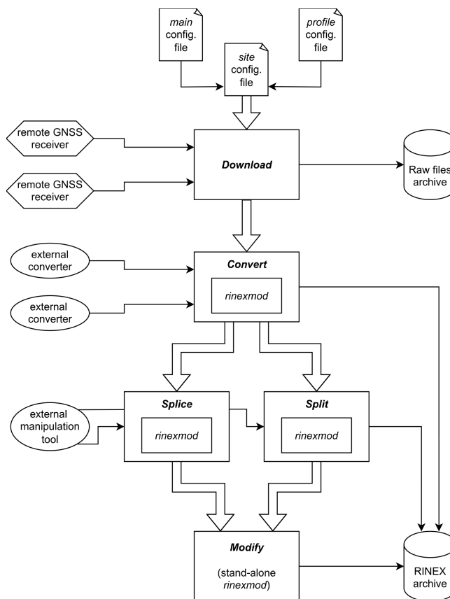
Figure 9. Standard workflow for autorino.
