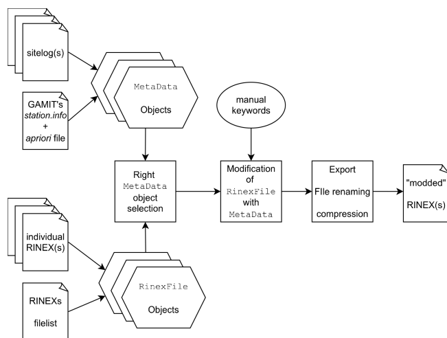
Figure 8. Standard workflow for rinexmod.
