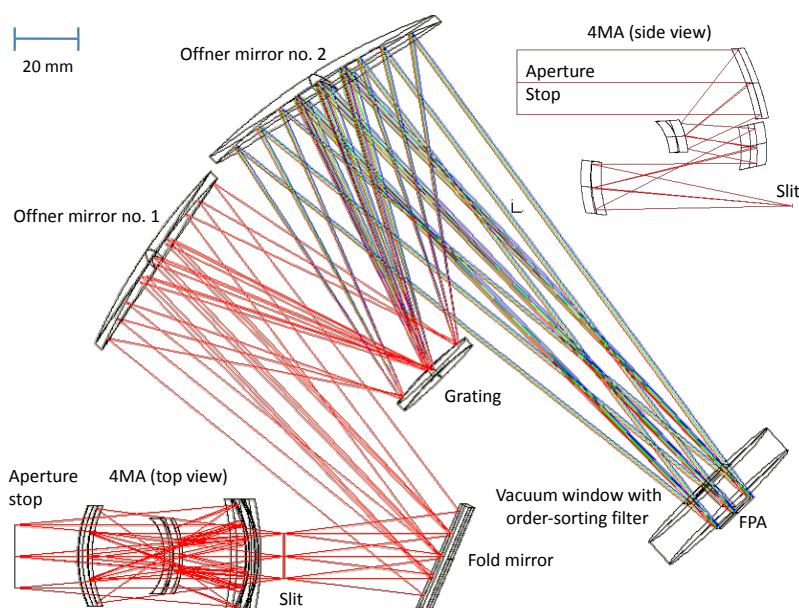
Figure 1. Optical layout of the HySICS shows the 4MA telescope followed by a grating-based Offner spectrometer that images onto a full-spectral-range HgCdTe focal-plane array with a three-region order-sorting filter on the back surface of its vacuum entrance window. The Offner and 4MA have nearly orthogonal optical-axis planes to reduce polarization sensitivity. The main picture shows a top view of the entire optical path, while a side view of the 4MA itself is shown in the upper right inset. The physical entrance aperture is positioned at the system's aperture stop. The spectrometer entrance slit is shown in its correct (albeit unconventional) orientation.
