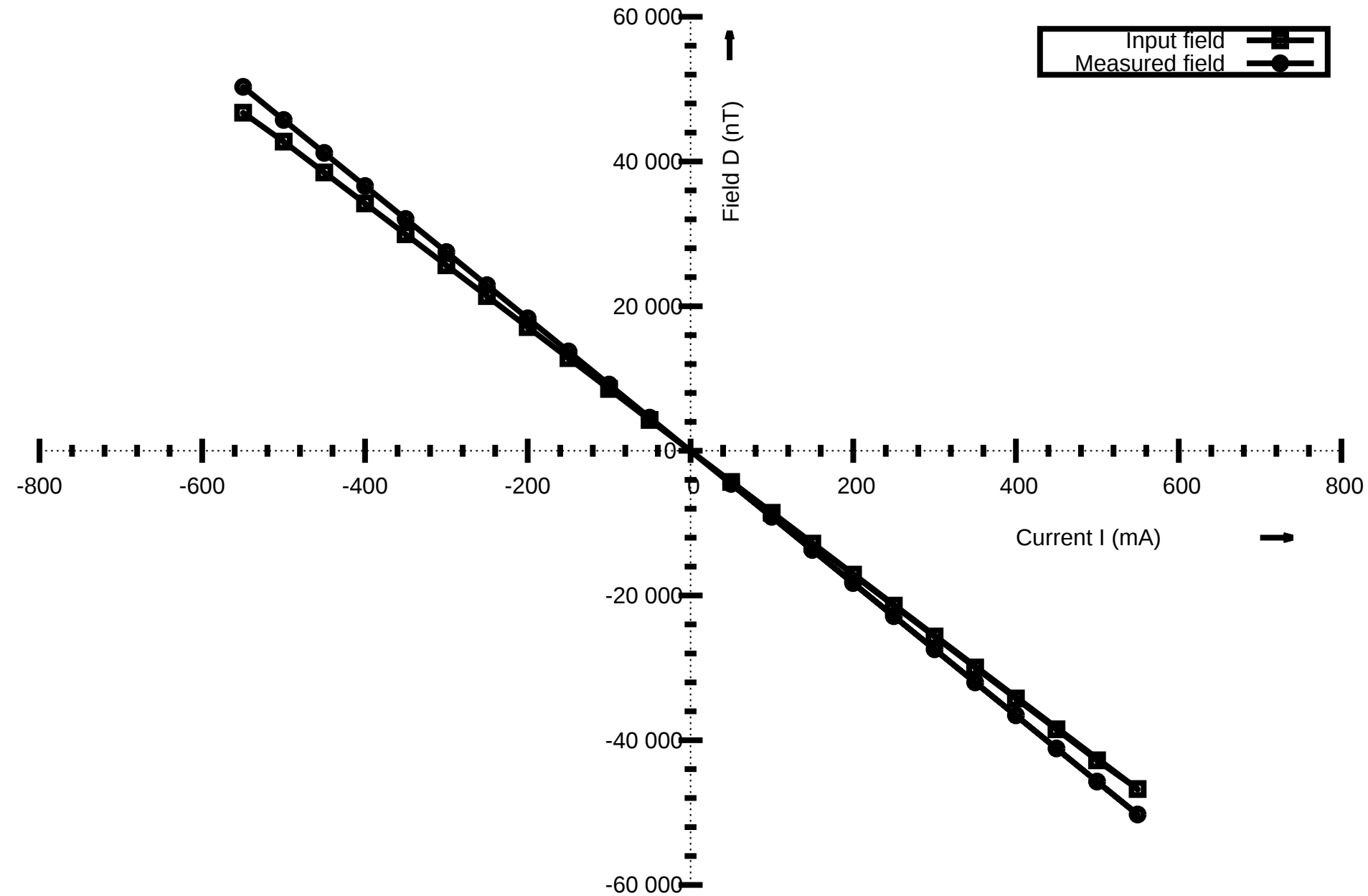
Fluxgate calibration sensor no. 1
