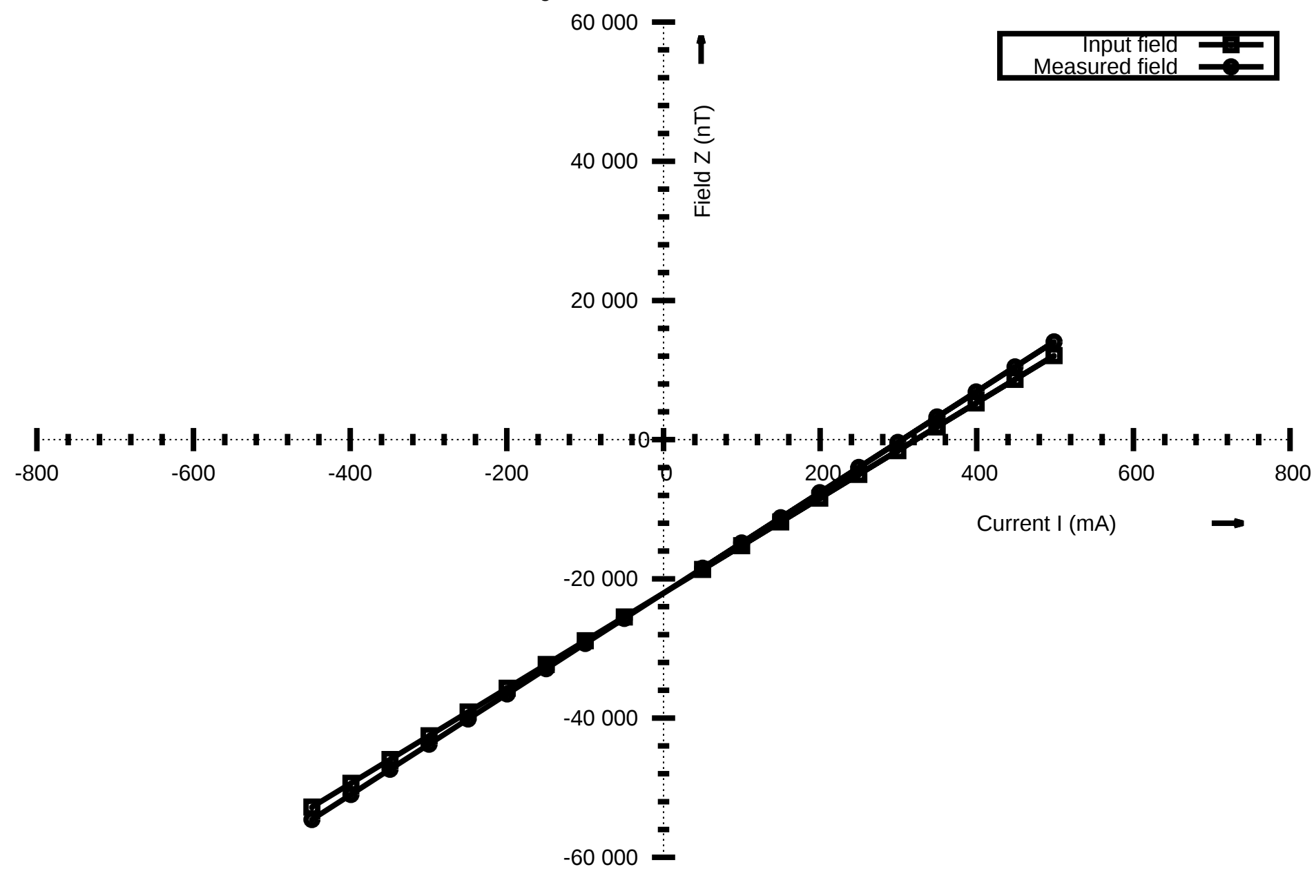
Fluxgate calibration sensor no. 1
