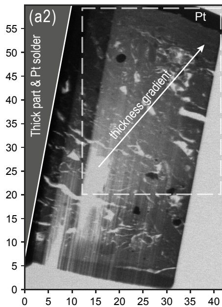
Mn pre-edge X-ray absorption
