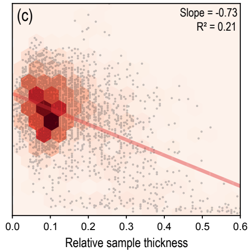
Manganese(II)-like cluster
