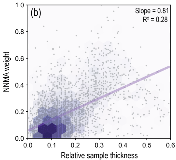
Manganese(IV)-like cluster
