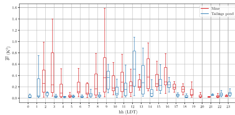
(e) Variance of potential temperature
