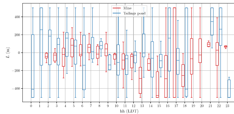
(c) Obukhov length
