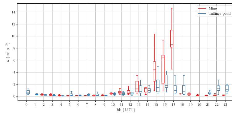
(a) Diurnal variation of turbulence kinetic energy
