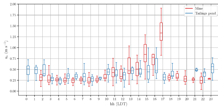
(b) Friction velocity
