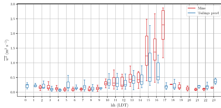
(f) Variance of vertical wind velocity
