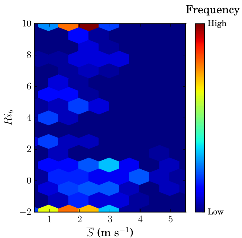
(b) Atmospheric dynamical condition near the tailings pond
