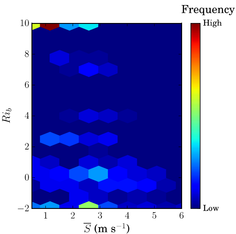
(a) Atmospheric dynamical condition in the mine
