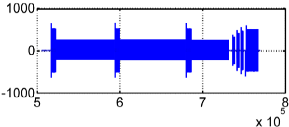
FFT of the data
