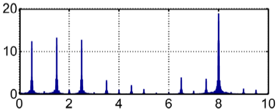
FFT of the data
