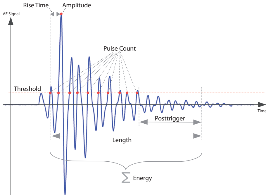
Fig. 1. Extracted parameters from AE signal.
