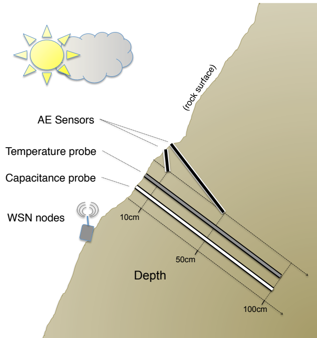
Fig. 8. Skematic view of the field setup of the measurement system.
