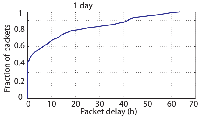
Fig. 12. CDF of packet delays, for packets generated by the two AE-Nodes. More than 80 % of all packets are forwarded to the network sink in less than 24 h.
