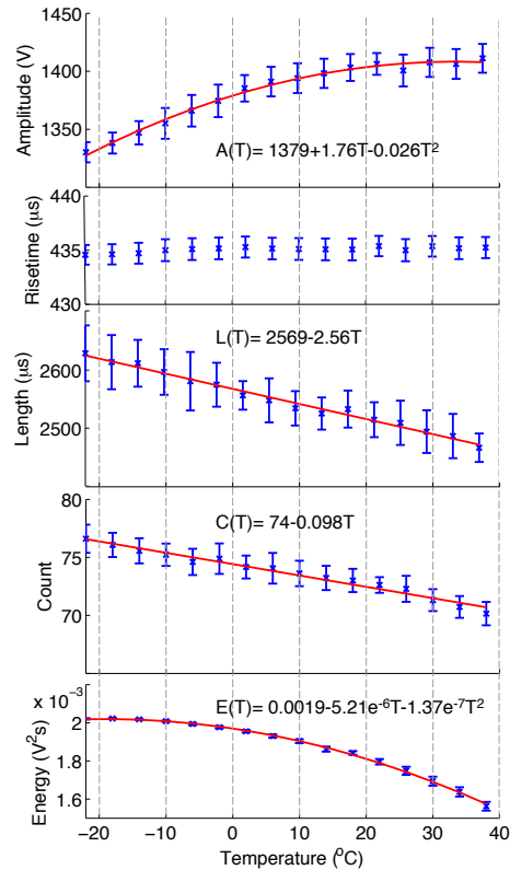
Fig. 3. Temperature dependency of measured AE signal parameters (mean and standard deviation) over a range from -20 to 40 °C. The risetime parameter remains stable whereas all other parameters show a noticeable temperature dependence. Linear regressions with respect to temperature ( T ) are given for the length ( L ) and count ( C ), while quadratic regressions are given for the amplitude ( A ) and energy ( E ).
