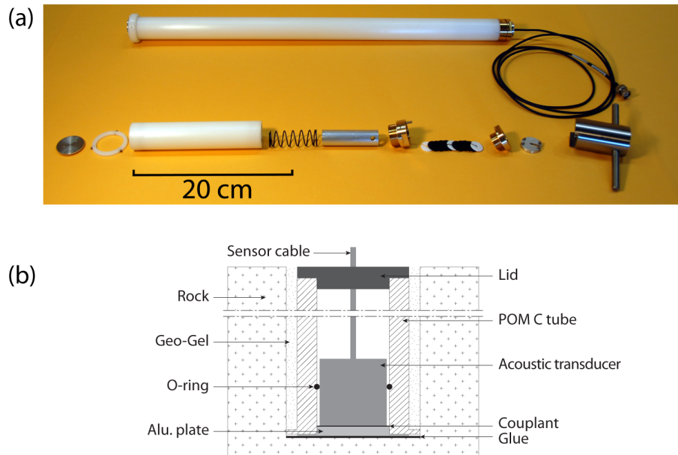
Fig. 4. (a) Picture of two copies of the AE casing, disassembled (bottom) and assembled (top), (b) Schematic view of the casing and acoustic transducer in a borehole.
