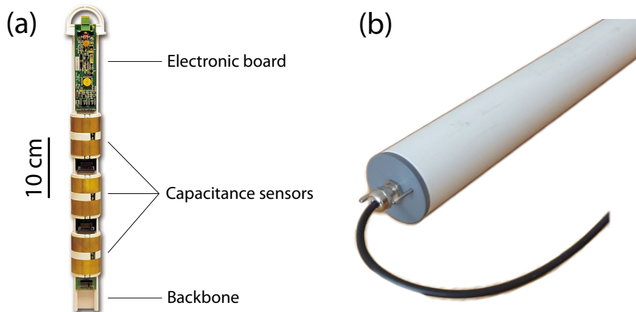
Fig. 6. (a) Capacitance probe EnviroSmart. The position of the electronic board and of sensors can be freely adjusted on the backbone, the setups used in our field deployments are described in Sect. 6. (b) Modified access tube.
