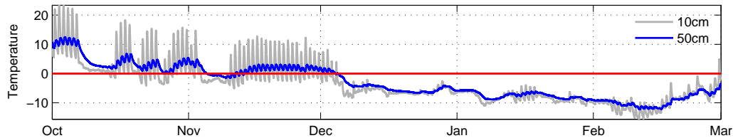
Fig. 9. Rock temperatures measured at M1.
