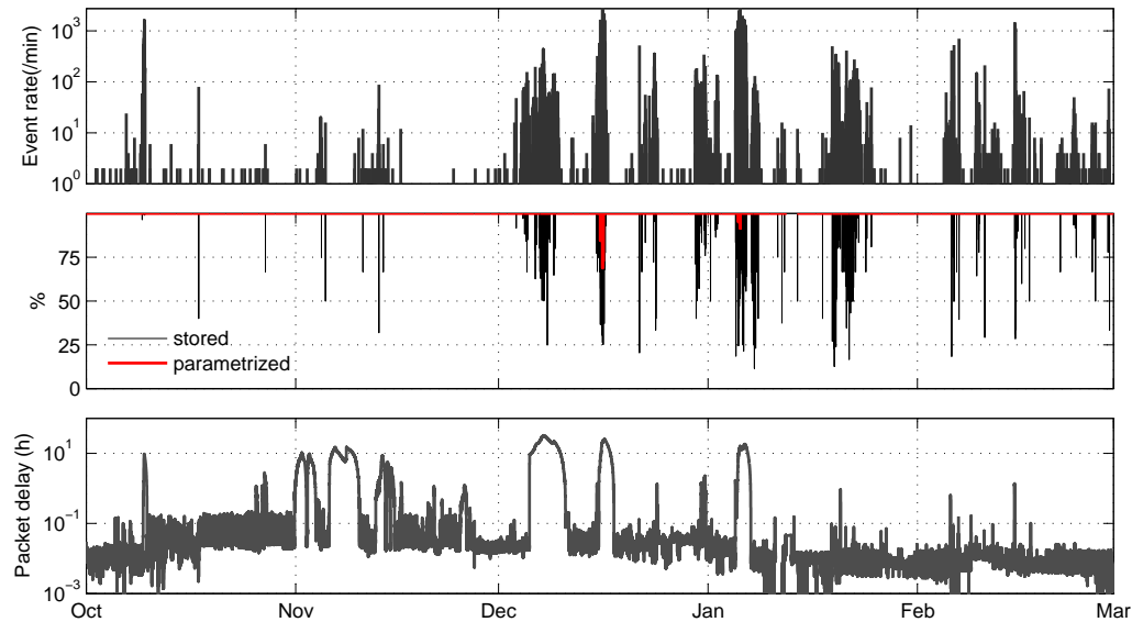
Fig. 10. Performance of the AE-node at M1: (a) rate of AE events measured, (b) percentage of all measured events that were parametrized, and fully stored (waveform), (c) time elapsed between generation of data packets and their transmission through the WSN.
