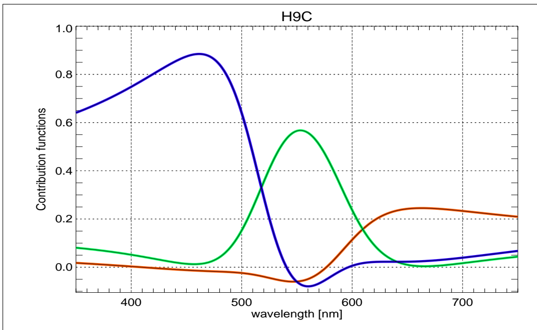
Fig. 10. Contribution functions ( D ) for the ICX285AQ with smoothing parameter \mu = 1 .
