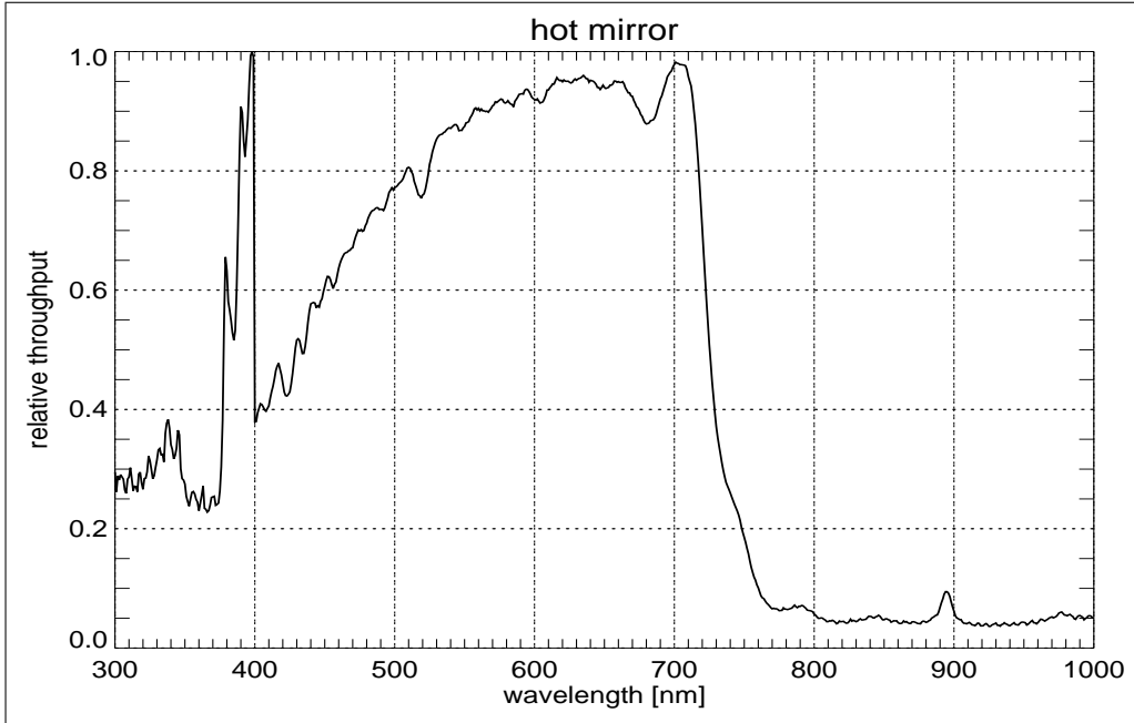
Fig. 9. Transmission for infra-red blocking filter (“hot mirror”) used in THEMIS and Rainbow cameras. Feature at 380–400 nm is a calibration artifact that does not significantly impact effect -analysis results.
