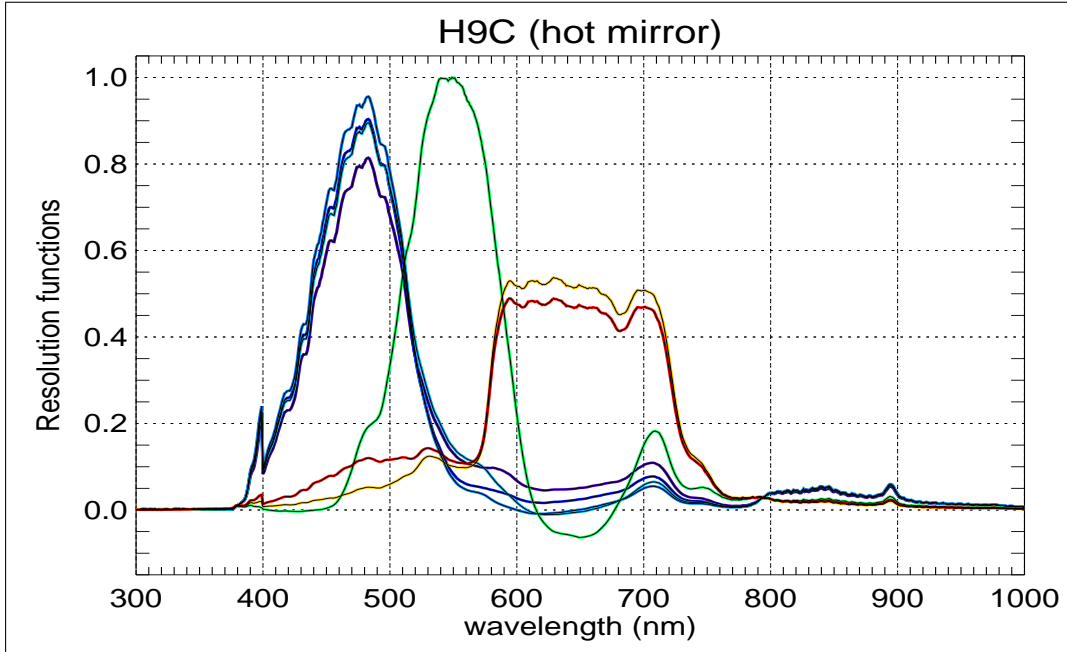
Fig. 11. Resolution/window functions ( A ) for ICX285AQ with smoothing parameter \mu = 1 and retrieved wavelengths of 391.4 nm (dark blue), 427.8 nm (blue), 470.9 nm (light blue), 486.1 nm (cyan), 557.7 nm (green), 630.0 nm (orange), and 777.7 nm (red).
