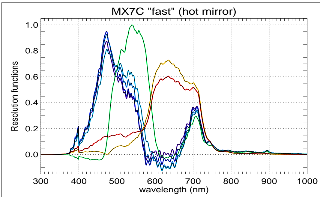
Fig. 13. Resolution/window functions ( A ) for ICX429AKL in “fast” mode with smoothing \mu = 1 and retrieved wavelengths of 391.4 nm (dark blue), 427.8 nm (blue), 470.9 nm (light blue), 486.1 nm (cyan), 557.7 nm (green), 630.0 nm (orange), and 777.7 nm (red).
