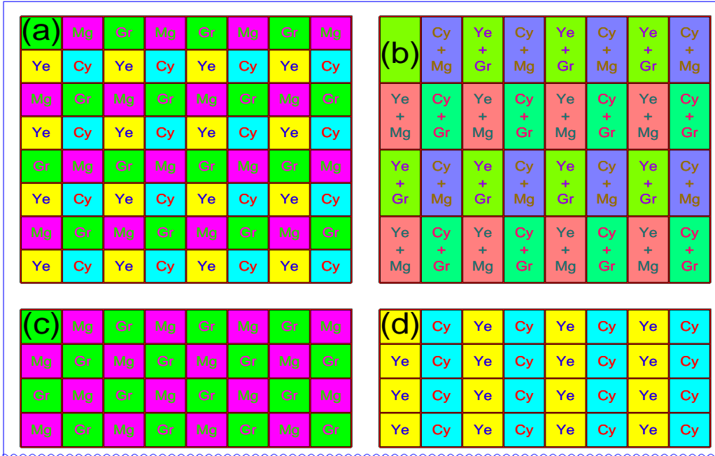
Sony ICX429AKL a) "raw" full color mosaic, b) "fast" binned row pairs, c) even rows, and d) odd rows.
