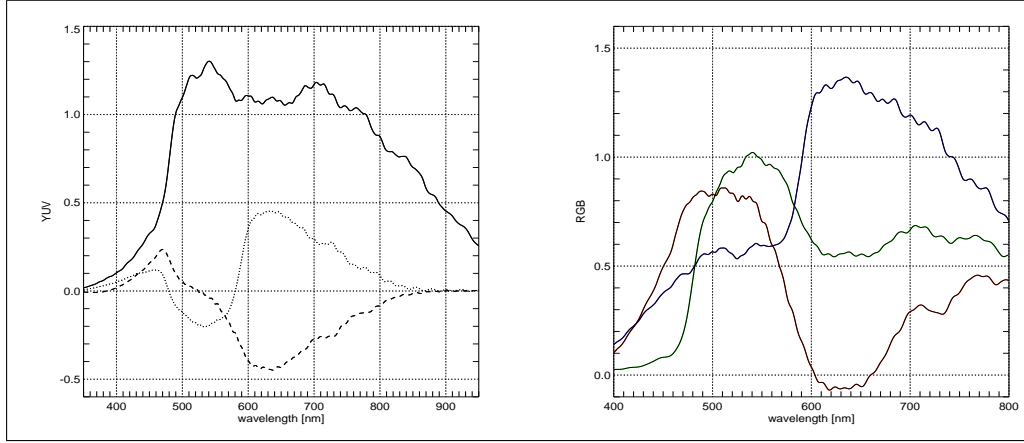
Fig. 25. Fast mode YUV (left) and RGB (right) spectral calibration (no hot filter).
