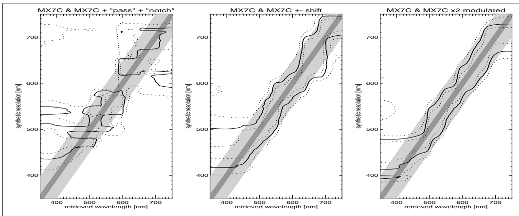
Fig. 21. Backus-Gilbert spectral response analysis for combinations of three color CCDs and filters: a) two different notch filters, b) two wavelength shifts of \Delta\lambda = \pm 9 nm, c) two sinusoidal modulations
