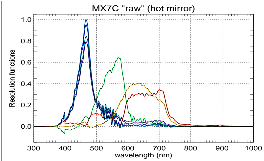
Fig. 14. Resolution/window functions (A) for ICX429AKL in “raw” mode with smoothing \mu = 1 and retrieved wavelengths of 391.4 nm (dark blue), 427.8 nm (blue), 470.9 nm (light blue), 486.1 nm (cyan), 557.7 nm (green), 630.0 nm (orange), and 777.7 nm (red).
