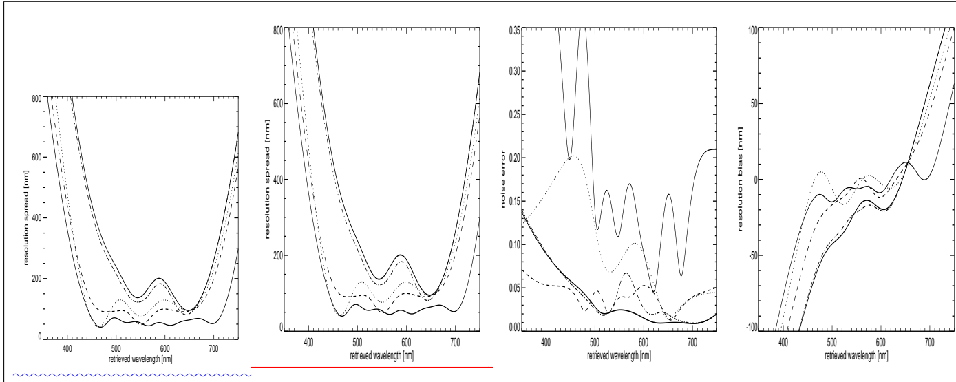
Fig. 22. Retrieval resolution ( q_2 ), noise, and bias ( q_3 ) for MX7C fast (thick solid line), MX7C raw (dotted), H9C/MX7C (dashed), 2\times MX7C with multi-notch filter (dash-dot), 3\times MX7C with two sinusoidal filters (thin solid).
