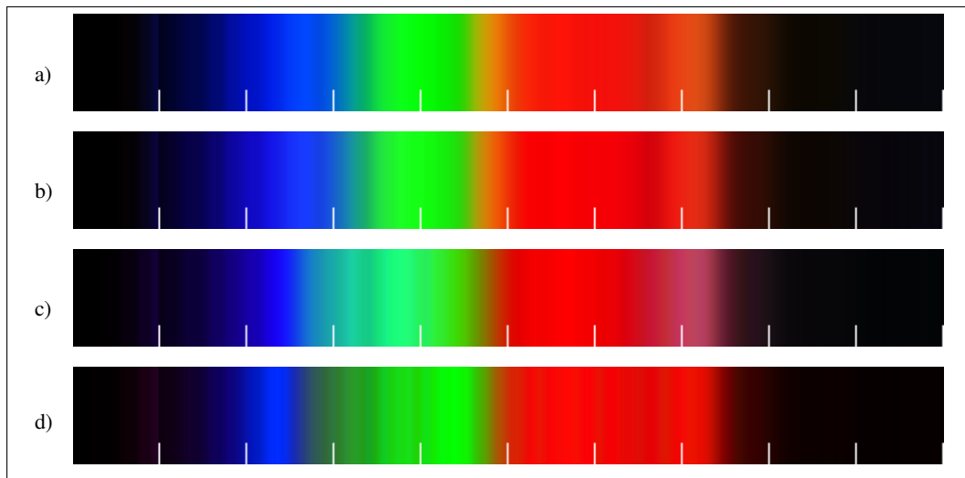
Fig. 17. Color bars for calibration wavelengths from 350 nm to 850 nm with tickmarks at 50 nm intervals. Top bar (a) is direct mapping of ICX285HQ Bayer matrix to RGB. Lower three are Backus-Gilbert estimation of CIE RGB channels for (b) ICX285HQ, (c) ICX429AKL fast mode, and (d) ICX429AKL raw mode.
