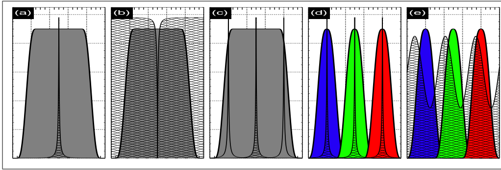
Fig. 19. a) broad-band CCD and narrow-band transmission filter, b) broad-band CCD and narrow-band rejection (“notch”) filter, c) broad-band CCD and 3 different narrow pass-band transmission filters, d) 3 channel wide-band color CCD and a single transmission filter with 3 narrow pass-bands, e) 3 channel wide-band color CCD and a single modulated transmission filter.
