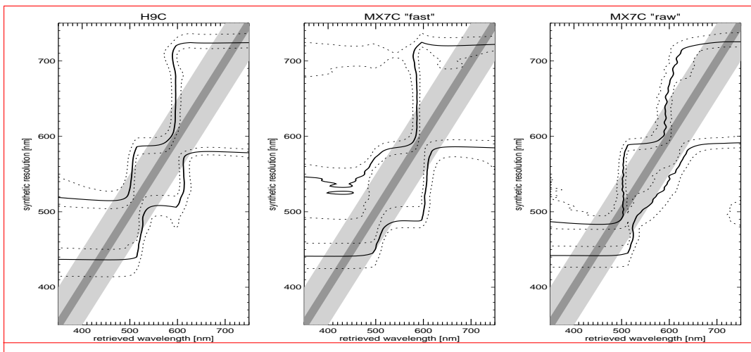
Fig. 12. Contour plots of resolution function (y-axis) variation with retrieved wavelength (x-axis). All functions are normalized to unit peak; full-width half-maximum (FWHM) is indicated by the solid contour. Light and dark diagonal shading corresponds to an unbiased detector with FWHM=100 nm and 20 nm respectively.
