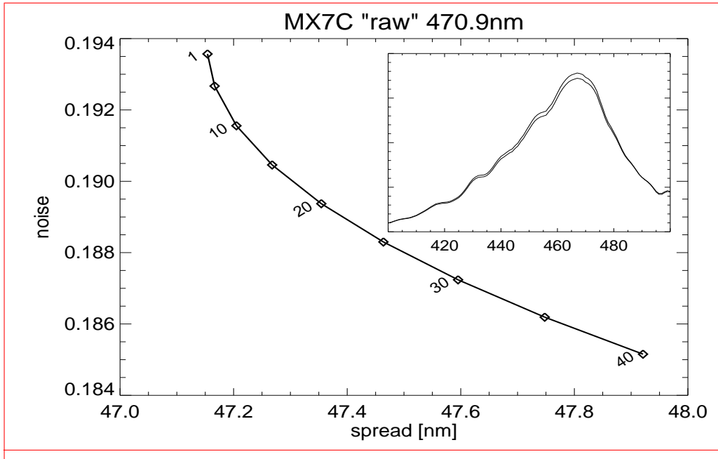
Fig. 15. Backus-Gilbert trade-off curve with inverse relationship between resolution function spread and retrieval error. Results were obtained using MX7C "raw" kernels with a retrieval wavelength of 470.9 nm and \mu ranging from 1 to 40. Inset shows nearly indistinguishable resolution functions for \mu = 1 and \mu = 40 .
