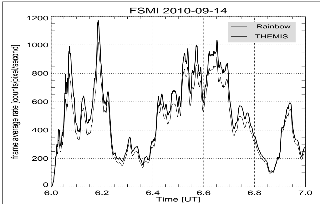
Fig. 8. Response of co-located Rainbow and THEMIS imagers at Fort Smith during an active period from 6–7 UT on September 14 2010. Frame average counts are divided by exposure times of 1 second for THEMIS and 5 seconds for Rainbow to produce comparable rates. THEMIS data ( thick line ) are plotted at 3 second intervals and Rainbow ( thin line ) at 6 second intervals; timing differences are not visible on this one hour interval. Results are very highly correlated ( r^2 \approx 0.994 ) with a ratio of 87%.
