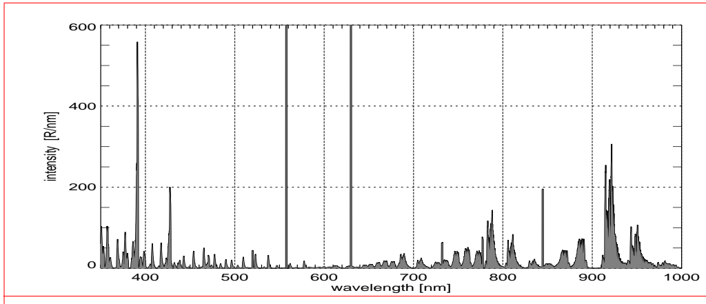
Fig. 1. Auroral spectrum during low activity geomagnetic and solar conditions for a beam of 1 keV monoenergetic electrons with a total energy flux of 1 milliwatt/m 2 . Intensity range is clipped to display spectral structure, 630.0 nm red-line peak is approximately 810 R/nm and 557.7 nm green-line is 1190 R/nm.
