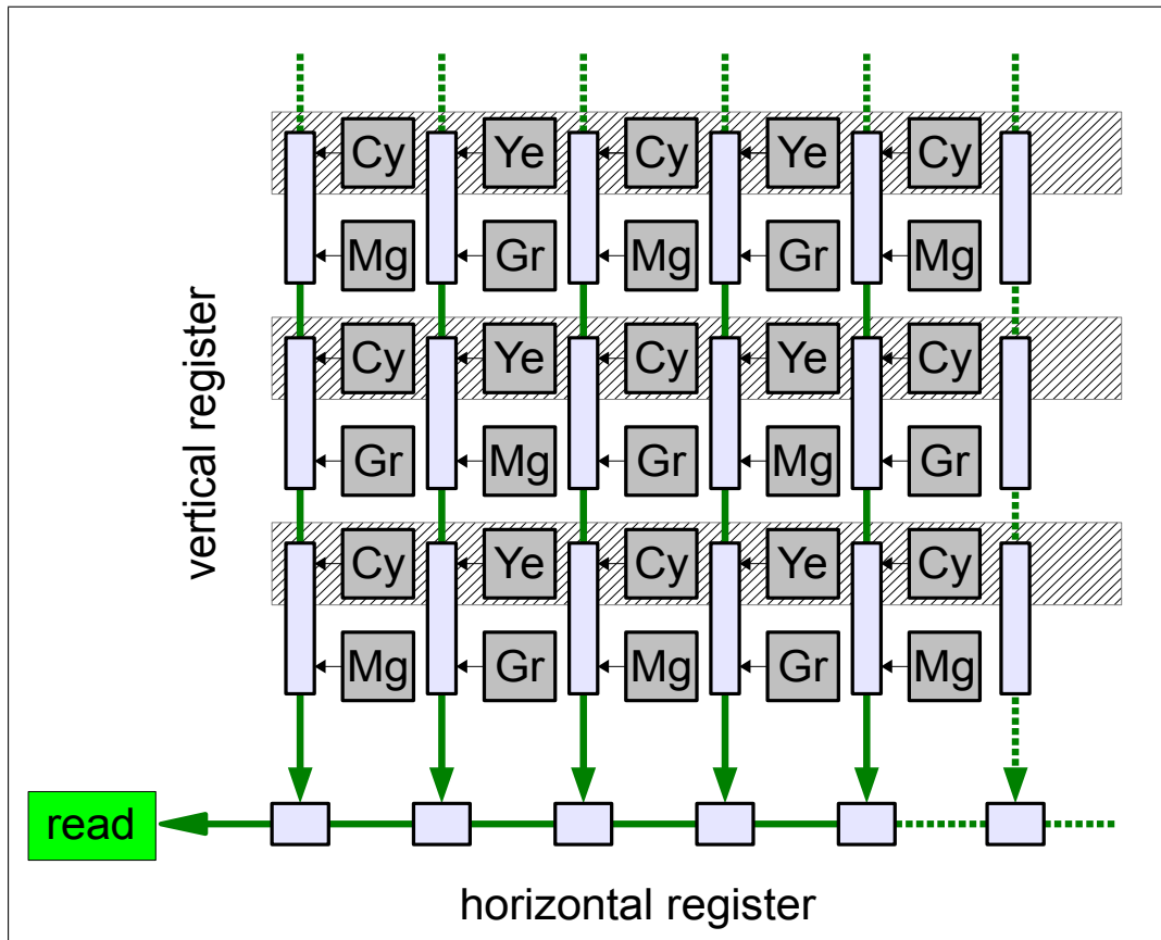
Fig. 23. Interline interlaced CMYG CCD geometry.
