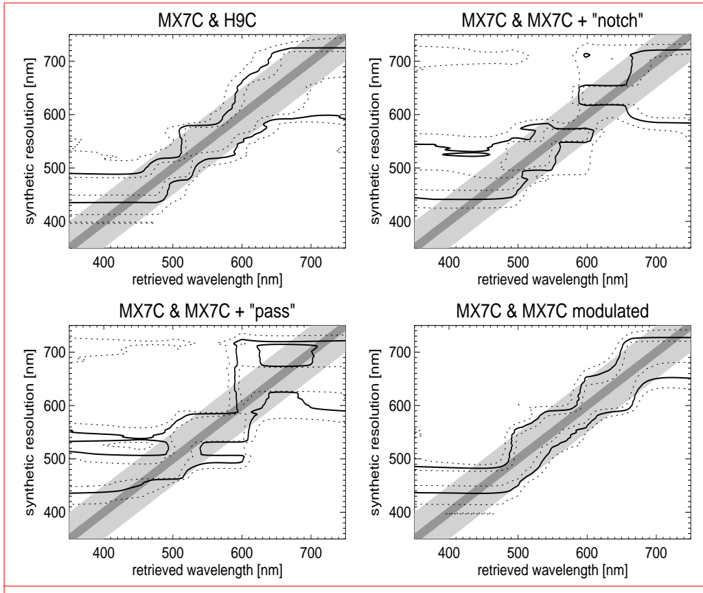
Fig. 18. Backus-Gilbert spectral response analysis for combinations of two color CCDs and filters.
