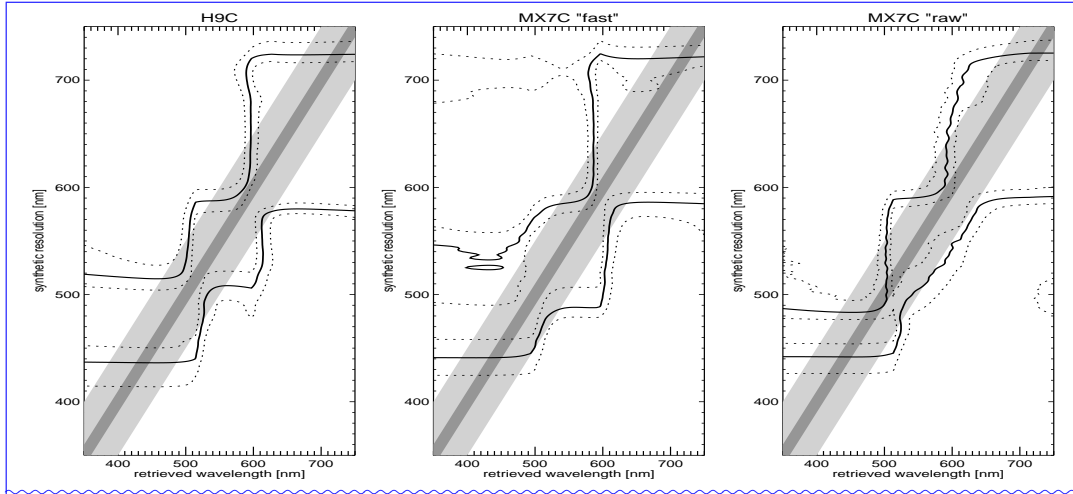
475 Contour plots of synthetic bandwidth (y-axis) variation with retrieved wavelength (x-axis). All functions are normalized to unit peak; full-width half-maximum (FWHM) is indicated by the solid contour. Light and dark diagonal shading corresponds to an unbiased detector with FWHM=100 nm and 20 nm respectively.
