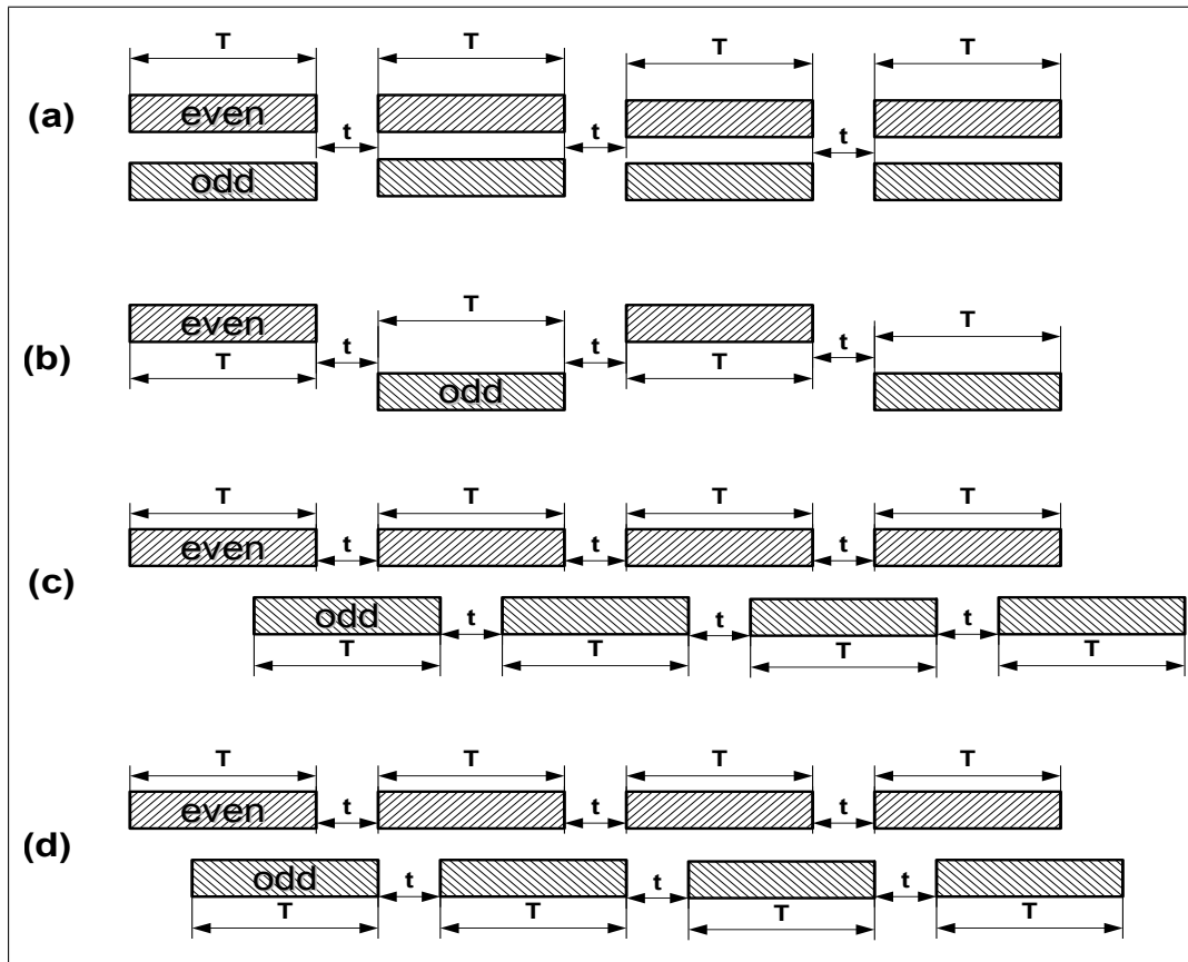
Fig. 24. Timing for interlaced read-out: a) “fast-mode” with combined simultaneous even and odd rows, b) alternating non-overlapping even/odd, c) alternating overlapping offset, d) “pseudo-progressive” alternating minimal offset.
