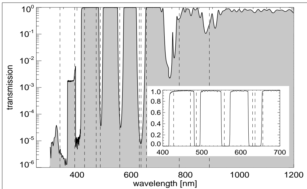
Fig. 20. Spectral transmission for a Semrock NF01-405/488/561/635 multi-notch filter with rejection bands near 405 nm, 488 nm, 561 nm, and 635 nm. Vertical dashed lines correspond to some typical auroral emission wavelengths.
