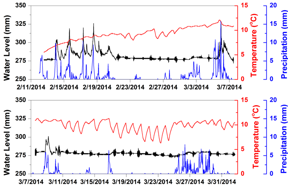
Figure 7. Long-term field monitoring data from the pressure transducer installed at Alesa site on Oregon Highway 34. The black, red, and blue lines represent water level, temperature, and hourly precipitation, respectively. The continuous monitoring was divided into two plots to show more details.
