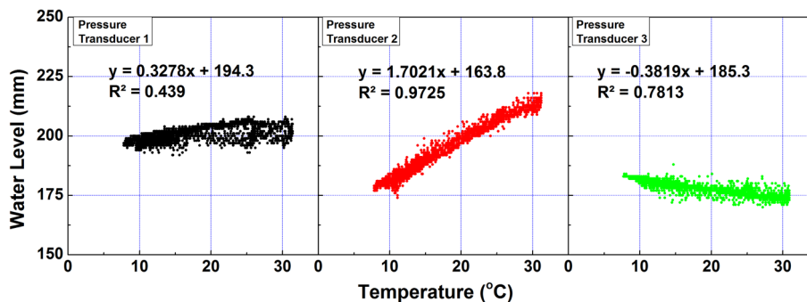
Figure 3. Relationships between temperature and water level readings.
