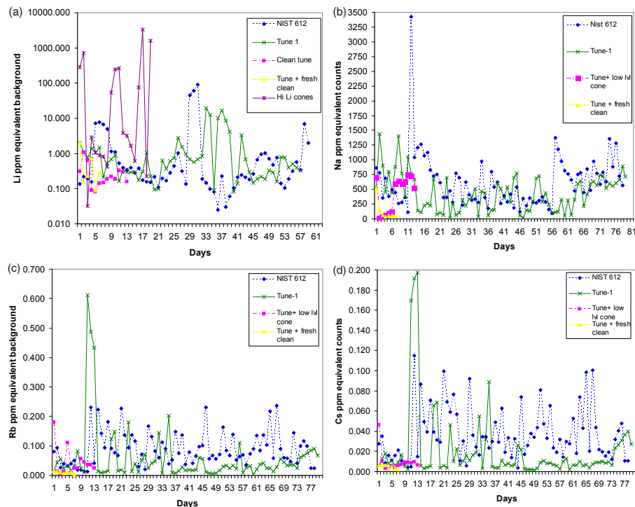
Figure 1. (a) Daily Li backgrounds as \mu\text{g g}^{-1} equivalent for high Li cones, standard cones tuned with NIST612, standard cones tuned with Tune-1, low level cones tuned with Tune-1, and freshly cleaned cones tuned with Tune-1. (b) Daily Na backgrounds as \mu\text{g g}^{-1} equivalent for tuning done with NIST 612, Tune-1, and Tune-1 with low level and freshly cleaned sets of cones for low level alkali work. (c) Daily Rb backgrounds as \mu\text{g g}^{-1} equivalent for tuning done with NIST 612, Tune-1, and Tune-1 with low level and freshly cleaned sets of cones for low level alkali work. (d) Daily Cs backgrounds as \mu\text{g g}^{-1} equivalent for tuning done with NIST 612, Tune-1, and Tune-1 with low level and freshly cleaned sets of cones for low level alkali work.
