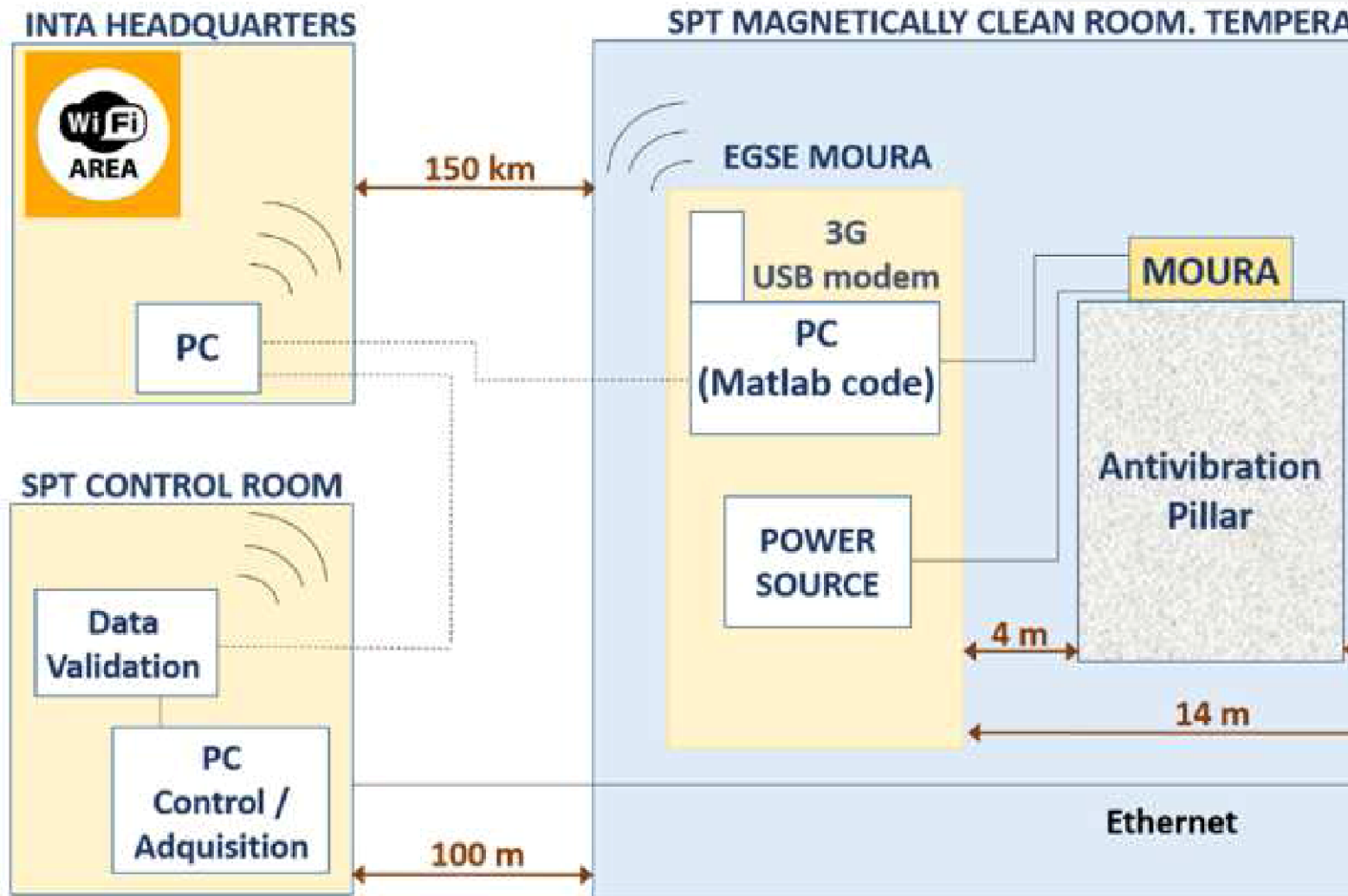
Fig. 2. Set up of the measurements.
