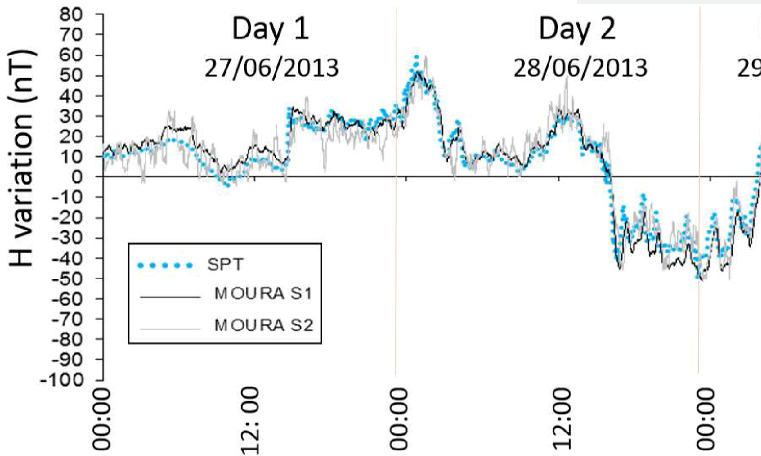
Fig. 4. Horizontal component of the geomagnetic field measured with MOURA magnetometer and SPT
