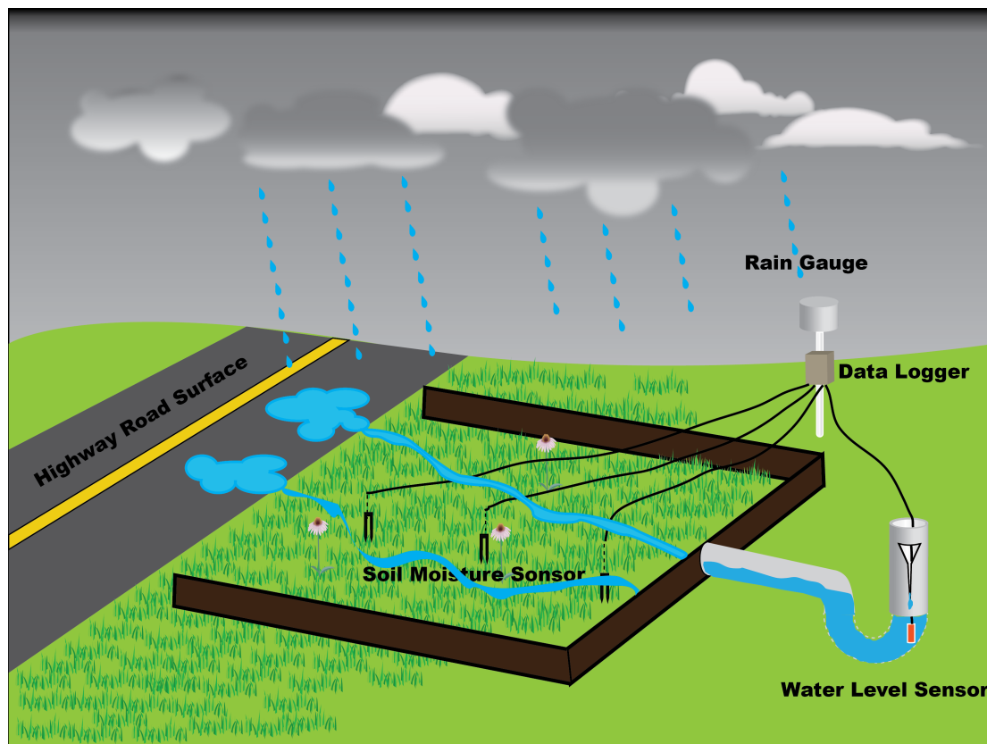
Fig. 1. A schematic of the field monitoring site.
