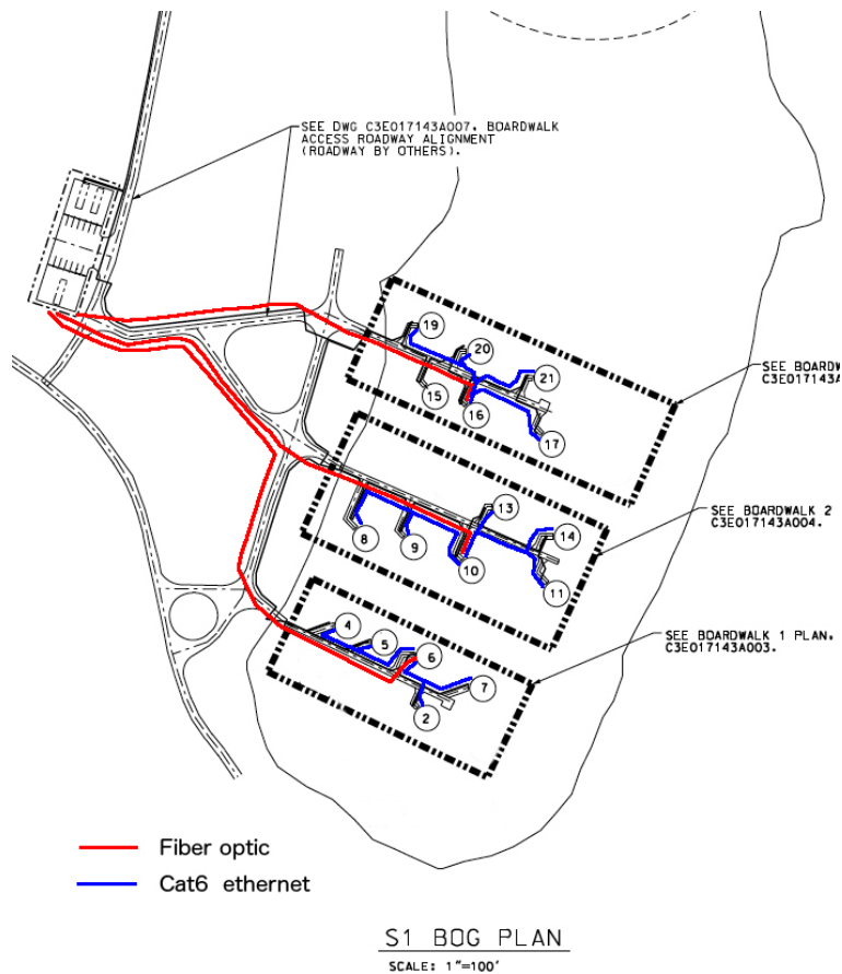
Figure 4. Network layout.
