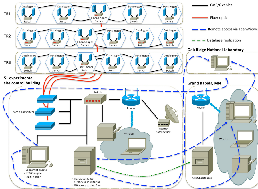
Figure 5. SPRUCE data collection and monitoring system.
