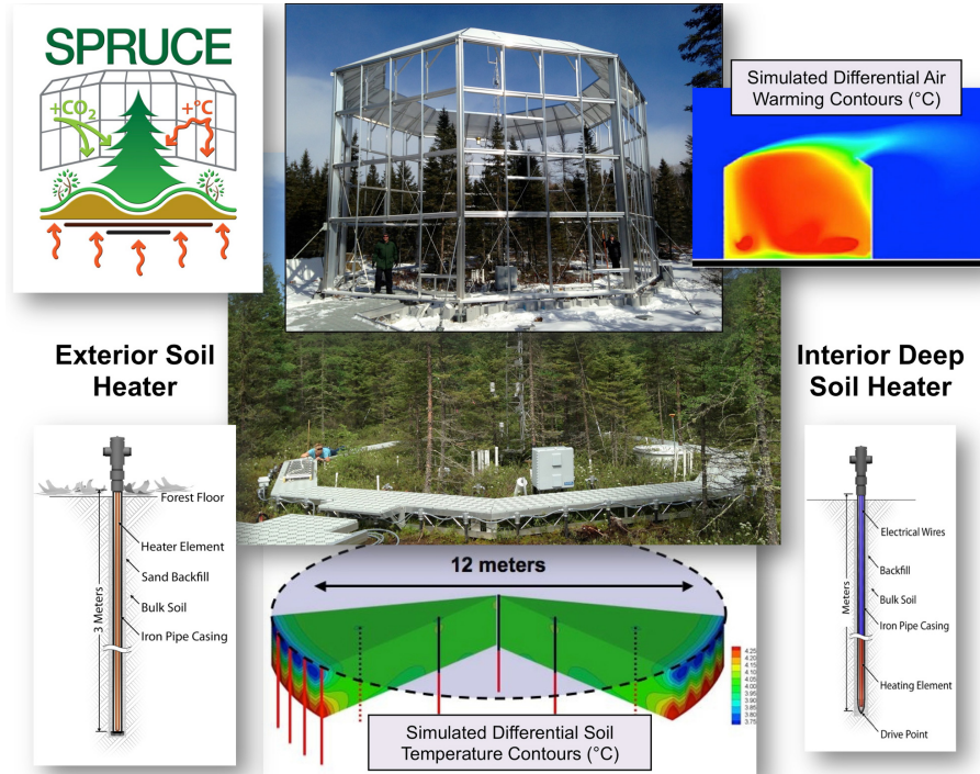
Figure 2. Open-topped enclosure on the S1-Bog for air warming of the peatland ecosystem.
