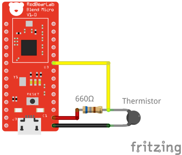
Figure 1. Schematic overview of the circuit used to readout the measurements from the thermistor.
