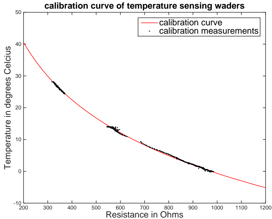
Figure 3. Results of the Calibration experiment, showing the resistance of the waders (x axis) vs. the temperature of the water as measured by TidBits (y axis). The red line is the fitted Steinhart–Hart relation.
