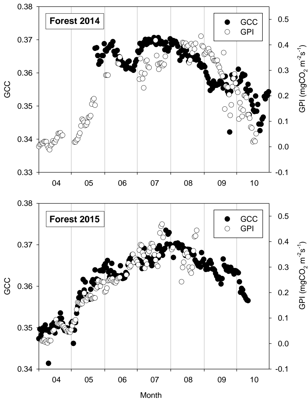
Figure S2: Mean daytime (11.00–15.00) GCC (crown camera) together with the gross photosynthesis index (GPI) at the forest site in a) 2014 and b) 2015.
