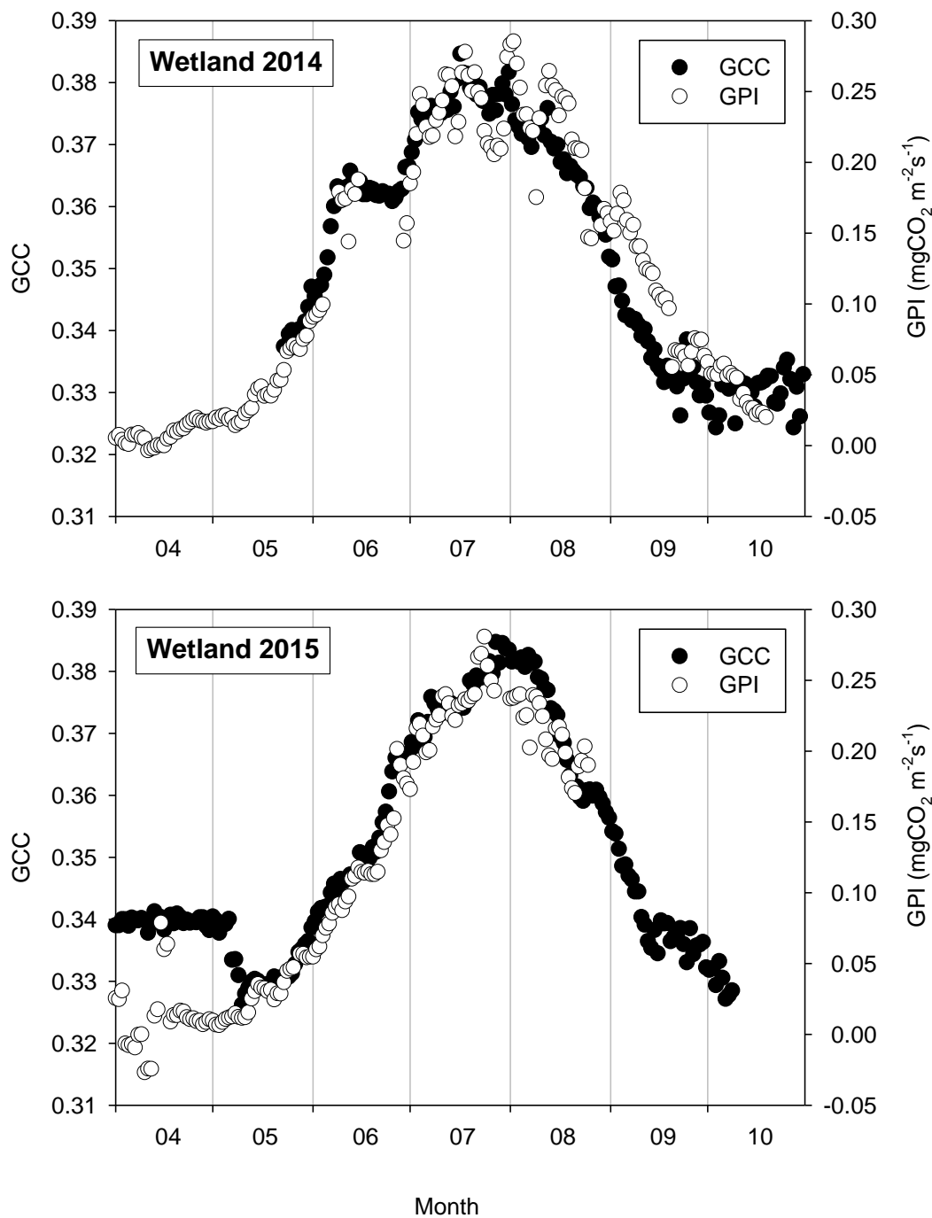
Figure S1: Mean daytime (11.00–15.00) GCC together with the gross photosynthesis index (GPI) at the wetland site in a) 2014 and b) 2015.
