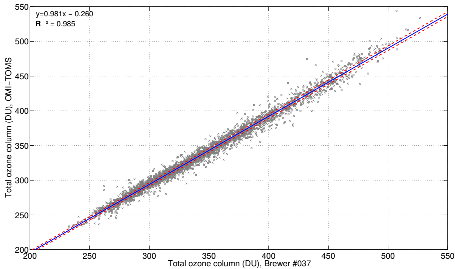
Figure 6. Comparison of Brewer #037 direct sun measurements and OMI satellite data using TOMS retrieval algorithm. The Brewer reference value was the closest direct sun measurement with a limit of maximum of one hour difference in the measurement times.
