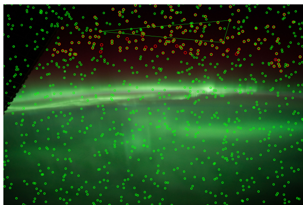
Figure 4. Results of applying astrometry.net to the image in fig. 1. Green circles represent the locations of catalogue stars, red circles stars that have been detected in the image and identified.
