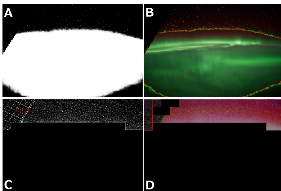
Figure 3. Stages of the automatic image masking process. A: The image is reduced to two colours to identify dark regions likely to be starfield. B: The resulting contour is applied to the original image. C & D: Image blocks not detected as starfield are masked and edge detection is applied to detect and mask linear features likely to be space station structure.
