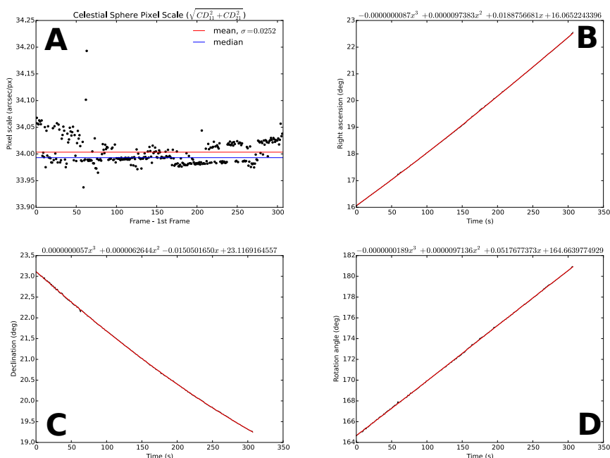
Figure 6. Astrometry parameters used for assessing the quality of a result. Figure 6A: The celestial sphere pixel scale for each image in a sequence (black) and its mean (red) and median (blue). Right ascension (6B), declination (6C) and rotation angle (6D) of the image centroid (black) and polynomial fits of each of these (red).
