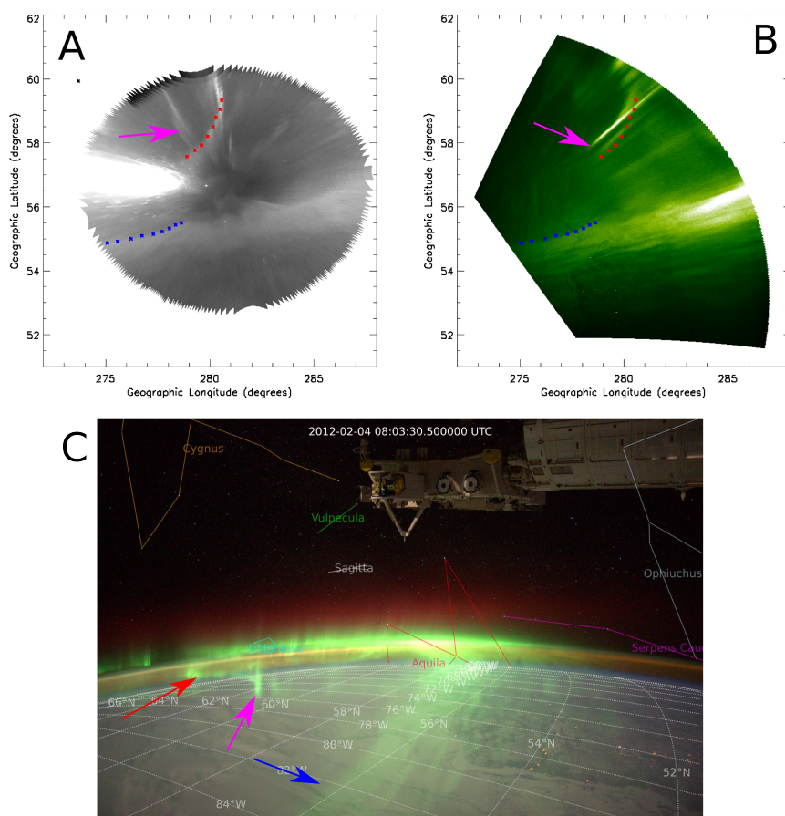
Figure 12. A more detailed comparison between the ISS image plotted in fig. 11 (Panel B) and the contemporaneous image acquired by the SNKQ THEMIS ASI (Panel A). The original ISS image is plotted in Panel C. Red and blue symbols trace the locations of the j shaped arc and northern edge of the main auroral arc, respectively, derived from their locations in the THEMIS image. The features are marked with the same coloured arrows in panel C. The magenta arrows point out a vertical feature projected very differently in A and B.
