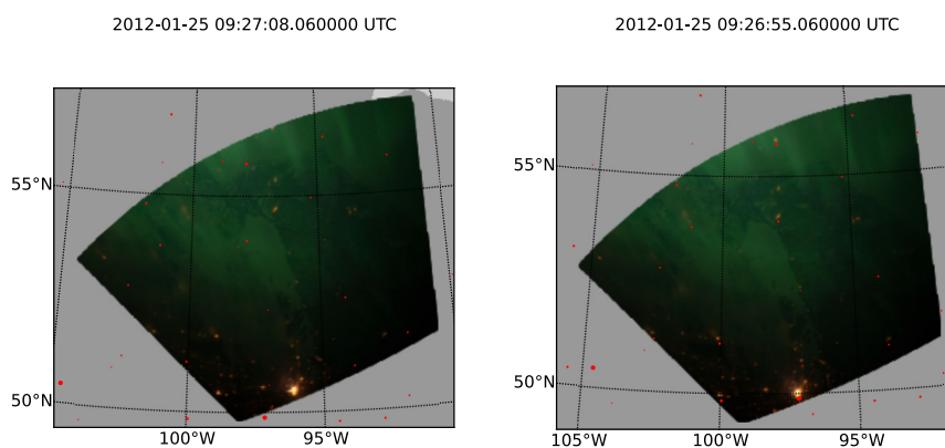
Figure 7. The left hand panel shows an image containing city lights projected to ground level rather than 110km, with the locations of cities overlotted in red. The right hand panel shows the same image when the timestamp has been corrected by 13 seconds to maximise agreement between the city lights and city locations.
