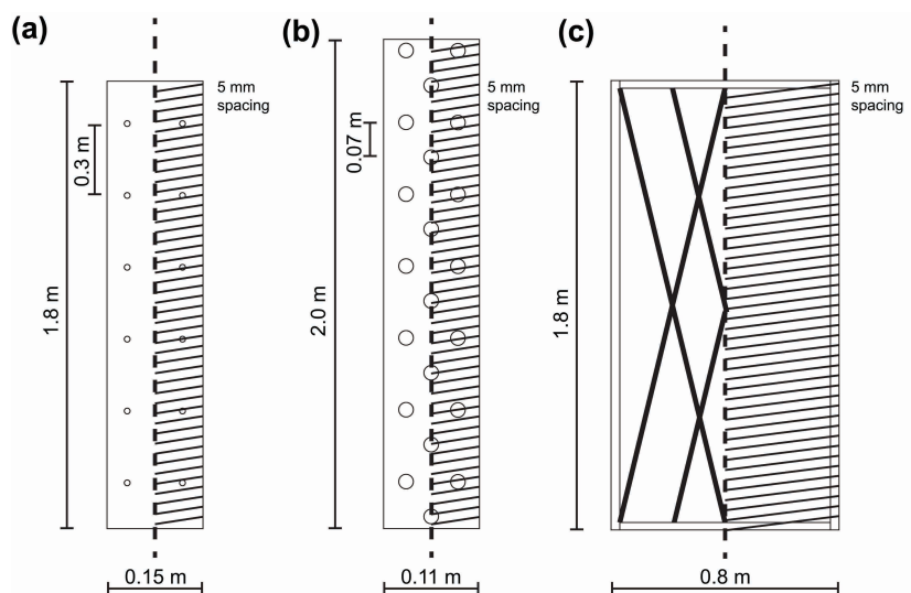
Figure 3. Measurement setups of the three experiments, (a) in Delft from 25 – 30 June 2012, (b) in Delft from 9 July – 7 August 2014, and (c) 23 – 27 October 2011.
