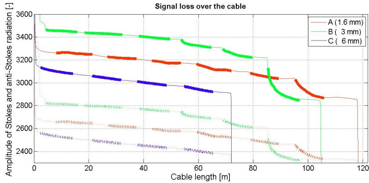
Figure 4. Amplitude of Stokes (solid lines) and anti-Stokes (dashed lines) radiation along the cables A (1.6 mm; red), B (3 mm; green), and C (6 mm; blue) when passing subsequent coils, marked by the thick sections of the graph. The coil diameters, from left to right, are 125, 75, 50, 32, 25, and 16 mm.
