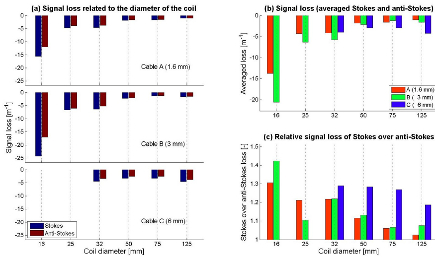
Figure 5. (a) Stokes and anti-Stokes signal loss ( m^{-1} ) for coil diameters of 16, 25, 32, 50, 75, and 125 mm, and for the cables A, B, and C (from top to bottom). (b) Combination of the bar plots in the left pane using the average of the Stokes and anti-Stokes signals. Loss decreasing with increasing diameter is indicative of bend-related light loss, which is generally associated with differential loss as a function of light frequency (c) Ratio of Stokes over anti-Stokes losses as a function of coil diameter.
