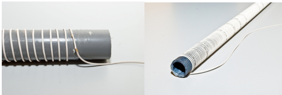
Figure 10. A damaged cable that was glued to a PVC conduit (left) and a cable wound through a furrow in the PVC conduit (right).
