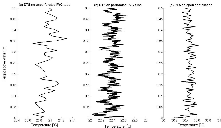
Figure 7. Typical air temperature profiles measured by DTS on (a) an imperforated PVC tube in Delft, (b) a perforated PVC tube and (c) an open construction. All profiles were taken on a cloudless day at 12PM.
