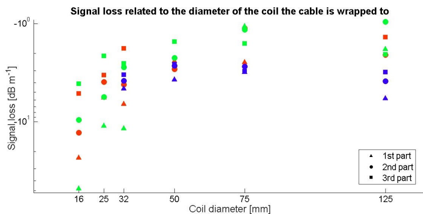
Figure 6. Signal loss ( \text{m}^{-1} ) over three subsequent sections of each coil presented for coil diameters of 16, 25, 32, 50, 75, and 125 mm, and for the cables A (blue), B (green), and C (red). The first, second, and third part each represent a third of the total coil length.
