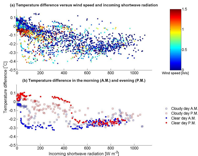
Figure 9. (a) Relation between temperature differences ( T_{\text{air}} - T_{\text{tube}} ), solar radiation, and wind speed (shown on colour scale in \text{m s}^{-1} ), (b) hysteresis in morning and evening transition in relation between temperature differences ( T_{\text{air}} - T_{\text{tube}} ) and solar radiation.
