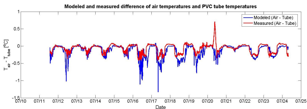
Figure 8. Measured (red) and modelled (blue) temperature differences between temperature measured over the holes and over PVC ( T_{\text{air}} - T_{\text{tube}} ) during July 2014 including a case of a morning dew on 20 July 2014.
