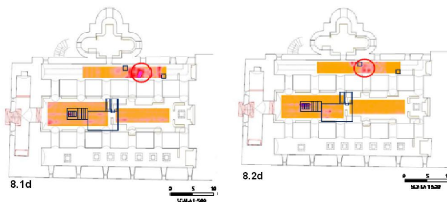
Slices at 65 ns: pulsed system (8.1d); stepped frequency system (8.2d)
