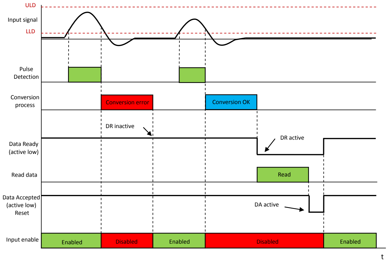
5 Figure 5. ADC conversion process. The ADC detects a peak when the input signal rises above the LLD threshold and below the ULD threshold. The detection process ends when the input pulse falls below 90% of its peak amplitude. In that moment, the signal input is disabled and the conversion process starts. If an error occurs in the conversion process, DR signal remains inactive and input signal enabled again. If conversion process is OK, DR is activated, the Data Acquisition System reads the data and activates DA signal, which causes the DA to go to inactive and the signal input to be enabled again.
