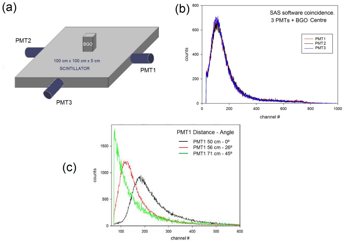
Figure 17. Software coincidence with four PMTs (MD2). Three of them placed in the sides of a 100 cm x 100 cm x 5 cm scintillator. The fourth one is set with a 6 cm x 2 cm Bismute Germanate scintillator (BGO). Coincident particle tracks pass through a relative small region of the large scintillator, just under the BGO. When moving BGO through the big scintillator surface, the histograms shift depending on the distance and the angle formed by PMT axis and the line between PMT and scintillator impact place.
