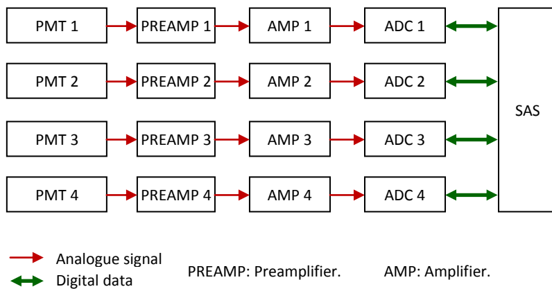
Figure 18. NIM modules and SAS interconnection block diagram working in software coincidence with four detection chains. The Signal from each PMT is amplified by preamplifier and amplifier in order to get the appropriate ADC input level. SAS detects coincidence and registers data.
