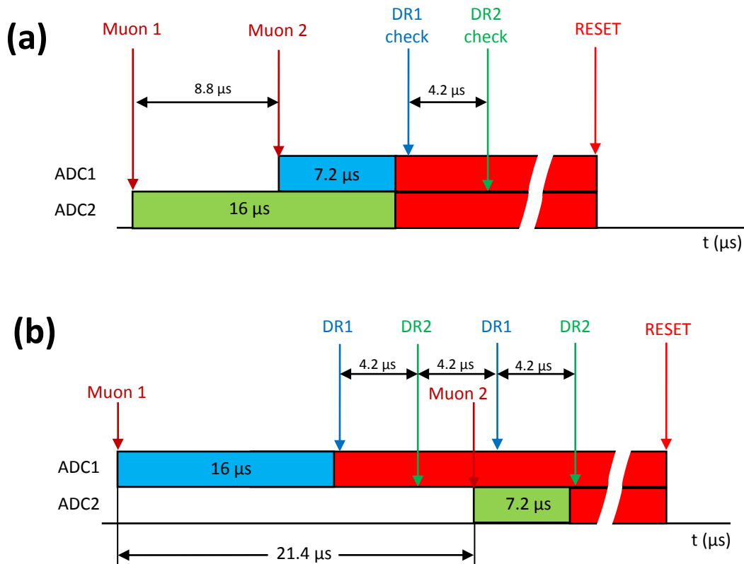
Figure 9. Different muons considered like a single particle (coincident) because of ADC conversion time (blue and green) and software checking time ( 4.2 \mu\text{s} between DR1 and DR2).
