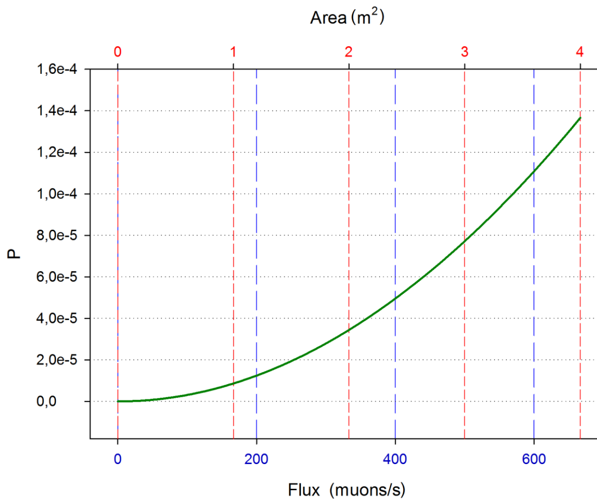
Figure 10. Poisson distribution. Probability of detecting as coincident two different muons in a period of \delta t = 25 \mu s as a function of muon flux (lower axis) or scintillator area (upper axis) at sea level.
