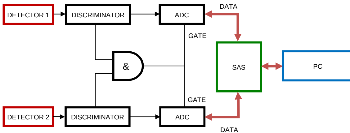
Figure 8. Hardware coincidence detector block diagram. The AND gate is the core of the circuit, its output become active when both inputs are activated. Here, the SAS only acquires and records data. It does not work as a coincidence system.
