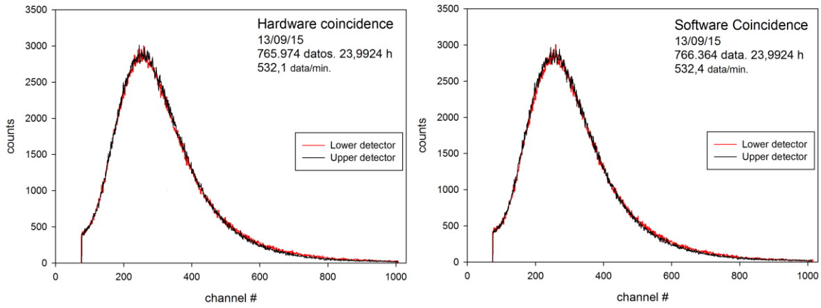
Figure 14. Comparative tests between data acquired with hardware (left) and software (right) coincidence by the muon telescope (MD1). Black and red lines correspond to the histogram of upper and lower detectors respectively.
