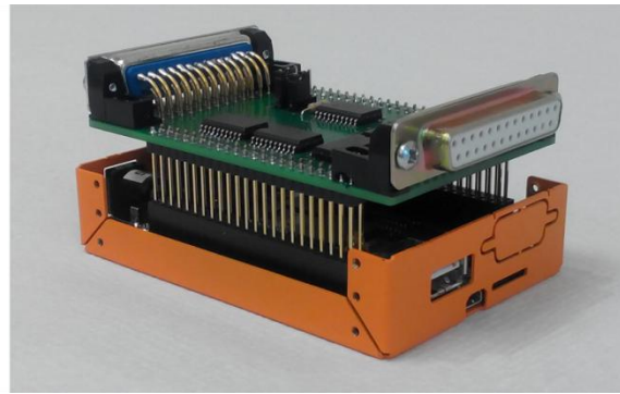
Figure 11. Left: Interface with two DB25 connectors. Right: Interface mounted on the process platform (Beaglebone Black) headers.
