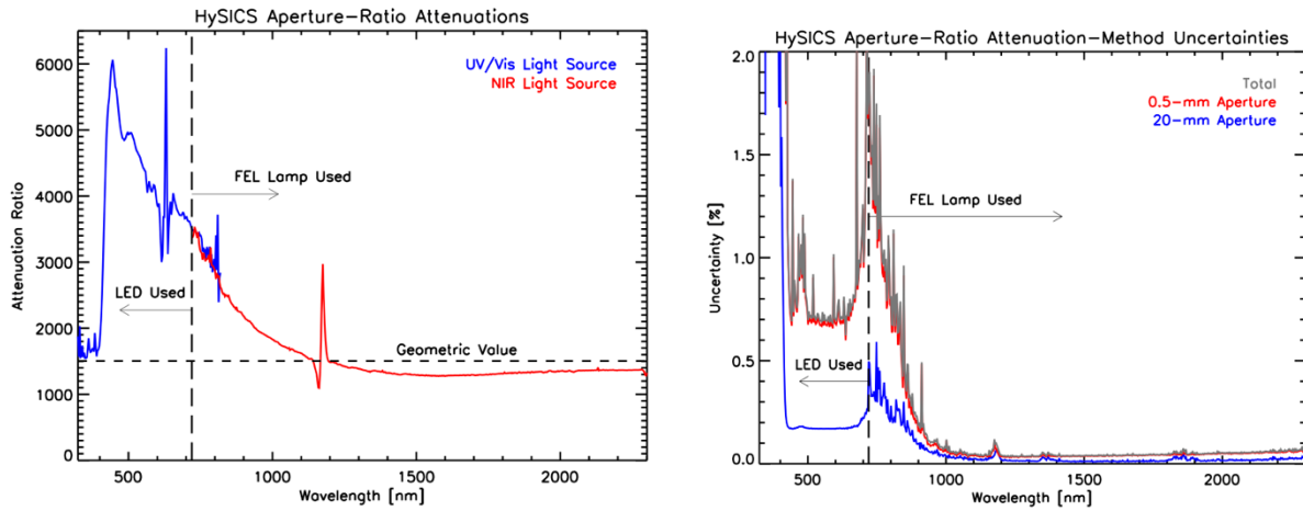
Figure 8: Different illuminations of the optical surfaces by the 0.5-mm and 20-mm apertures, mainly being affected by a boundary between grating blaze-regions, cause the spectrally-dependent attenuations that differ from the nominal geometric-ratio value due to the aperture-attenuation method, as shown in the left-hand plot. The blue and the red curves are based on different lab light-sources that provide peak power at shorter and longer wavelengths, respectively. The right-hand plot gives the uncertainties in these attenuations. The large peak in uncertainties between the two light sources used is due to low signals from each and could be improved with additional calibration light-sources.
