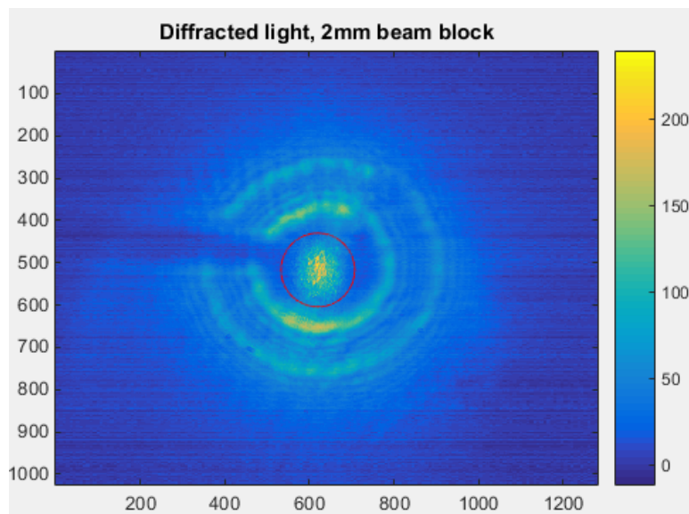
Figure 3: Lab scatter- and diffraction-characterization setup (upper schematic) gives the 2-D pattern shown in the lower image when using a 2-mm beam block behind the 0.5-mm solar-viewing aperture. This beam block occults the un-diffracted and un-scattered light incident on the aperture from a distant, nearly-collimated light source (left side of upper schematic). Most light that is diffracted or scattered by the aperture edges passes around the beam block to be reimaged onto the camera, helping quantify the intensity and spatial pattern of that light. The innermost Airy rings from typical aperture-edge diffraction are visible in the lower image. Since incident sunlight will diffract and scatter similarly, thus spreading some light beyond the edges of the solar-disk image, these effects must be corrected when determining net solar-irradiance values via spatial integrations from HySICS's cross-slit scans of the solar disk. Lab measurements such as these combined with diffraction models to account for wavelength sensitivity and extend the spatial extent help reduce uncertainties for those corrections. (The nearly-horizontal radially-extending dark region to the left of image center in the lower image is due to the support for the beam block.)
