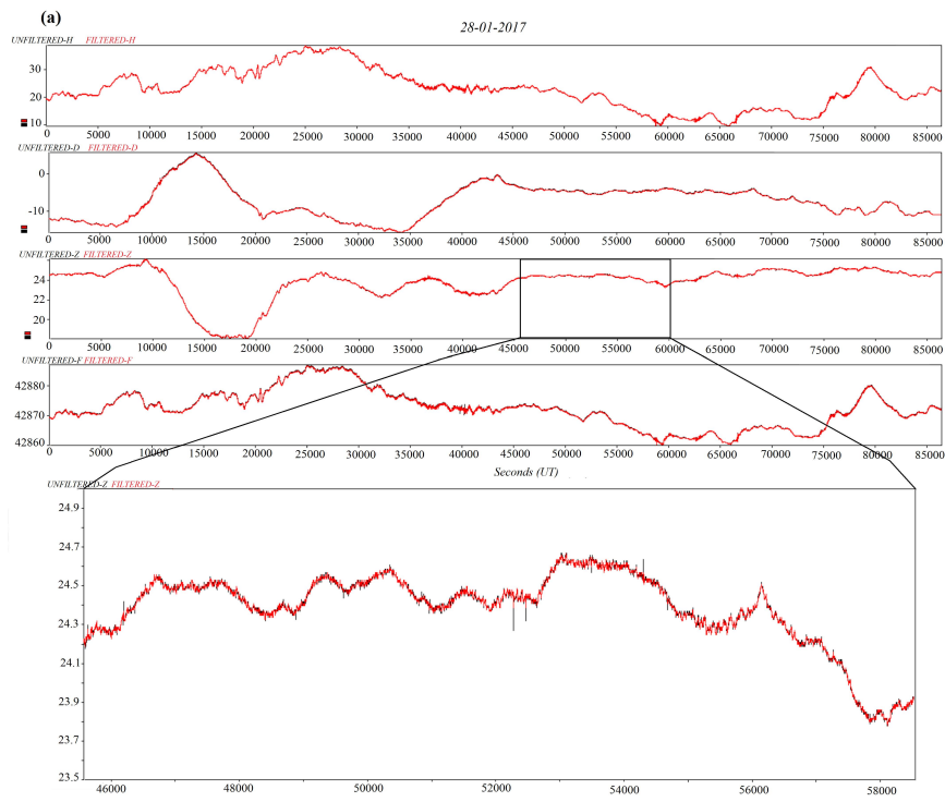
Fig. 4. Figure 9a. Sample plots of 1 second raw (black colour line) and filtered data (red colour line) with cut-off frequency 0.2 Hz from the CPL Magnetic Observatory.
