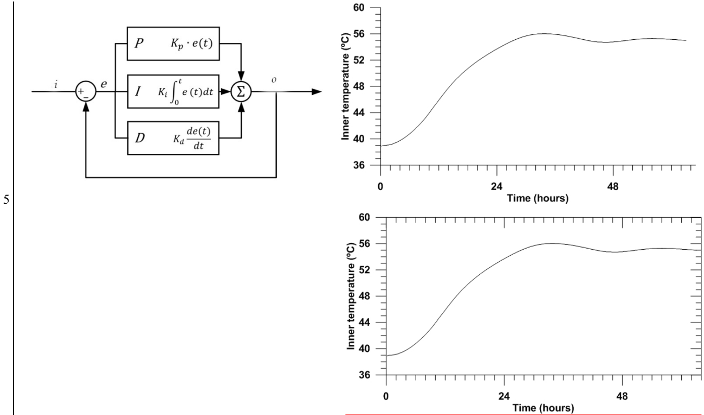
Figure 5: (a) Scheme of a PID controller showing its three components: proportional (P), integral (I) and derivative (D). The error, e , is the difference between the desired value, i (set point), and the achieved one, o . (b) Effect of the PID control on the box. Rise is observed up to the working temperature (set point of 55 °C in this case), followed by an oscillation which, in steady conditions, is about 0.3 °C in a 1-day period (test at Ebre Observatory).
