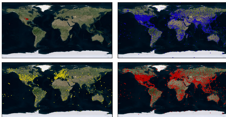
15 Figure 6: Classification based upon primarily “Uncertainty” MSMM category scores of the existing networks at the global scale providing in-situ water vapour measurement; upper left panel shows water vapour networks classified as “Comprehensive”; upper right panel, the networks classified as “Baseline”; lower left panel, the networks classified as “Reference”; lower right panel finally shows all the networks measuring water vapour at once. In this realisation, networks measuring the vertical profile, the full column
