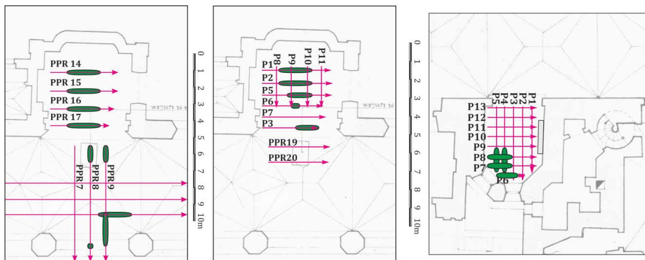
Figure 3. (a) Ground floor plan of the Dead's People Chapel with profiles set by 500 MHz antenna.(PPR 14, PPR 15, PPR 16, PPR 17). (b) Ground floor plan of the Dead's People Chapel with profiles set by 800 MHz antenna. (P1, P2, P3, P5, P6, P7, P8, P9, P10, P11). (c) Ground floor plan of the Chapel of St. Jacob with profiles set by 800 MHz antenna. (P1 – P5 & P6 – P13). Visualization thanks to the Department of Geophysics, AGH University of Science and Technology.
