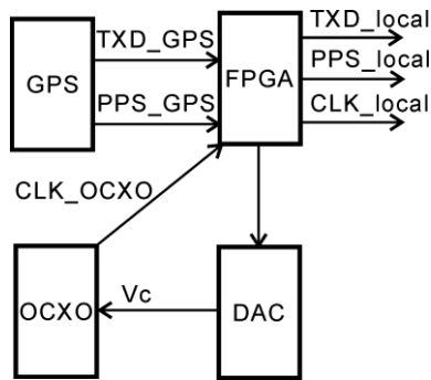
Figure 4. Block diagram of the clock module
