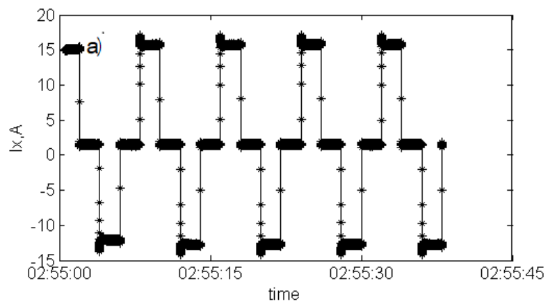
Figure 8 a) Raw current time series with whole circulation (15 min) and b) time frequency spectrum (SIP mode)
