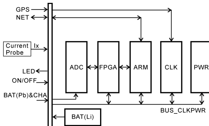
Figure 1. a) Diagram of multifunction EM transmitter architecture, b) picture of the transmitter (diesel generator, AC/DC regulator chopper module, current probe, data acquisition unit, cable, tablet computer (PAD))
