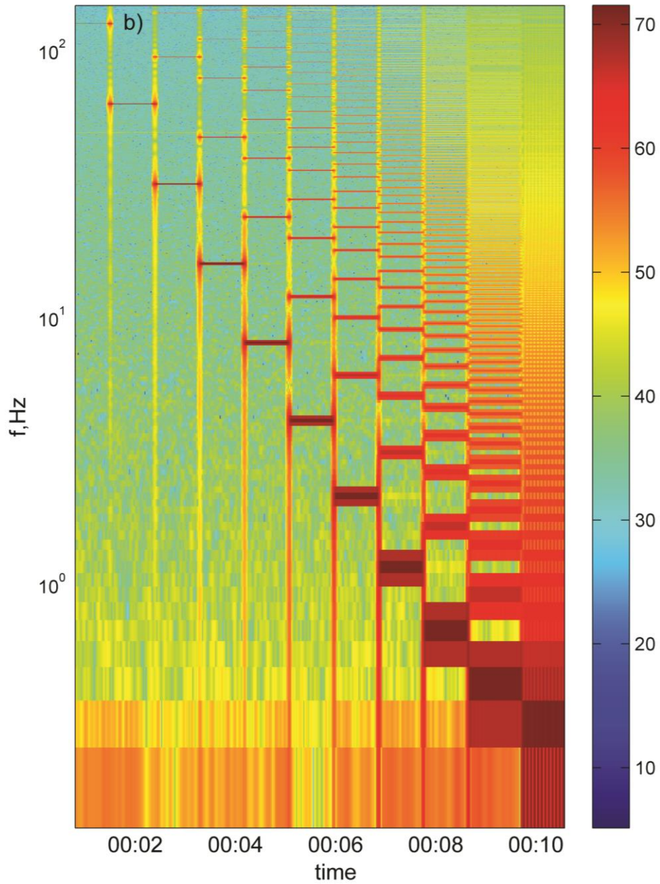
Figure 8 a) Raw current time series with whole circulation (15 min) and b) time frequency spectrum (SIP mode)
