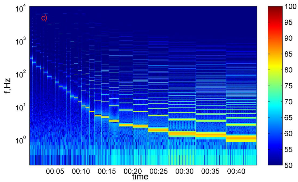
Figure 7a) Current time series as one complete cycle (CSAMT mode, duration 50 min, 9600 Hz to 0.9375 Hz, 2 Ap to 30 Ap); b) frequency stack result; and c) time frequency spectrum (CSAMT mode)
