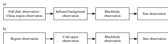
Figure 4: Time blocks for AGRI and GIRS used in daily operation: (a) AGRI and (b) GIRS.
