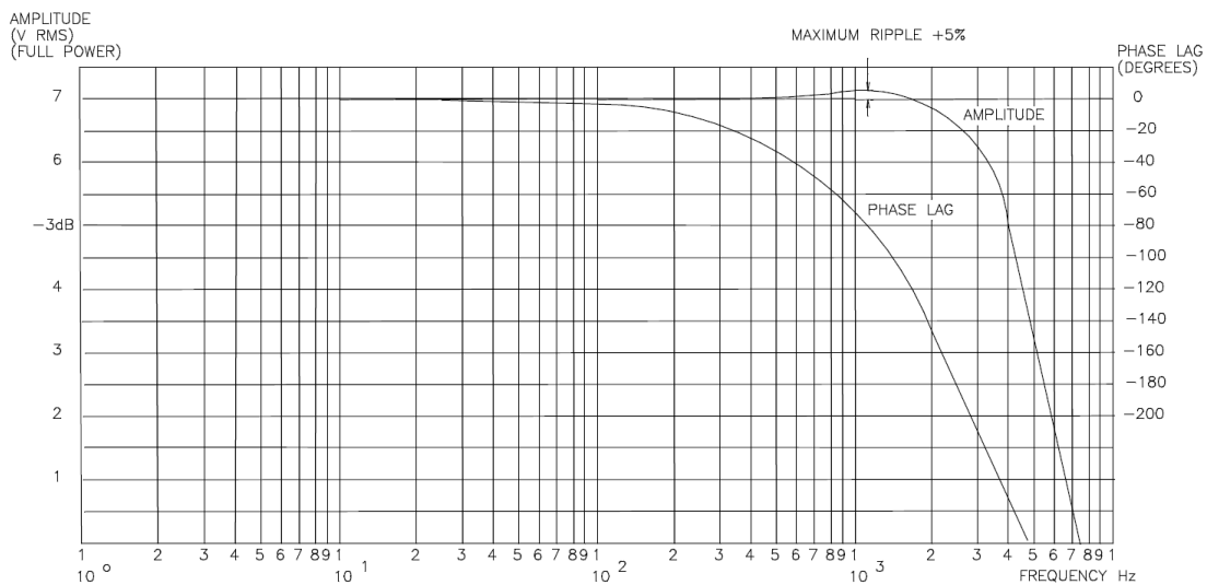
Fig. 1. Response of fluxgate
