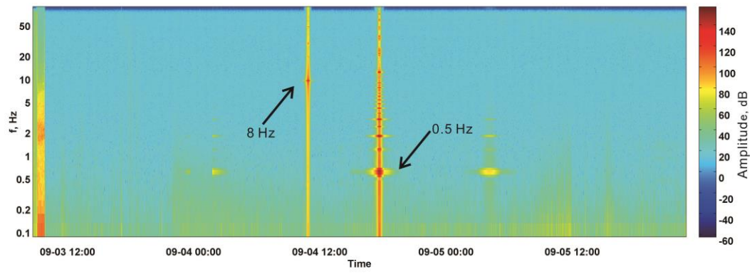
410 Fig. 7. Short time Fourier transform results for the CSEM signal from the horizontal electrical field components.
