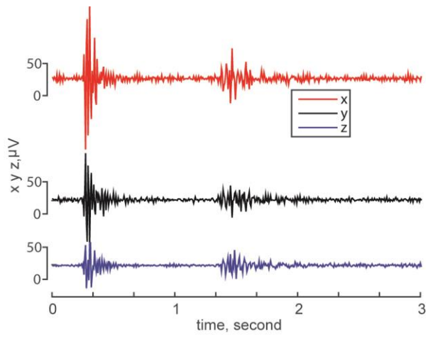
Fig. 9. Seismic data acquisition test results in real environmental conditions from the OBEMS at test site R21. (a) First horizontal component, (b) second horizontal component, and (c) vertical geophone component.
