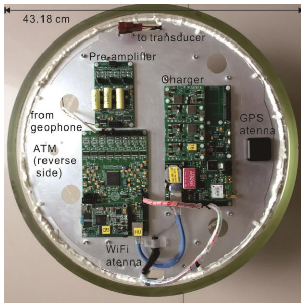
395 Fig. 4. Photo of the data logger installed in the glass sphere. Under the aluminum board, an ATM, Li-ion rechargeable battery set, and three-axis geophone are fixed. After circuit assembly, magnetic shielding covers the three print circuit boards to decrease sensor disturbance.
