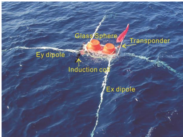
Fig. 2. Photograph of the OBEMS while in the water ascending to the surface after release. The length of the electrode dipole is 12 m.
