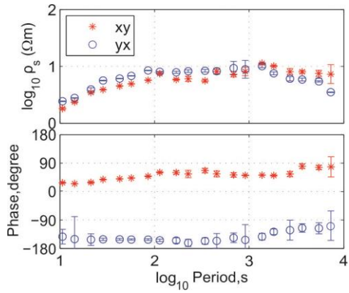
405 Fig. 6. Apparent resistivity (top) and phase (bottom) curves calculated from the OBEMS E-field and B-field at site R19. The red star indicates the xy component and the blue circles indicate the yx component.
