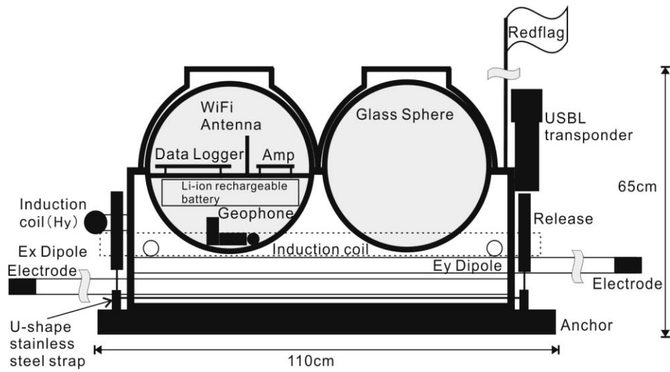
Fig. 1. Schematic diagram of the ocean bottom electromagnetic receiver and seismometer (OBEMS). Diagram shows the structural design inside the glass sphere, with omni-directional geophones in the lowest layer, followed by the Li-ion rechargeable battery packs, Acoustic Telemetry Modem (ATM), and the data logger. All print circuit boards are covered with magnetic shielding. Ferrite sheets, with a 0.01-mm-thick film on one side and a 0.02-mm-thick adhesive tape on the other, were glued inside the shielding box. These ferrite sheets function primarily as suppressors, blocking EM noise at lower frequencies and absorbing it at higher frequencies. A single U-shaped stainless steel strap connects the two release mechanisms, passing through two stainless steel loops set into the anchors.
