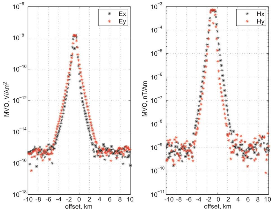
Fig. 8. Magnitude versus offset for the E and H components (site: R19, frequency: 8 Hz).
