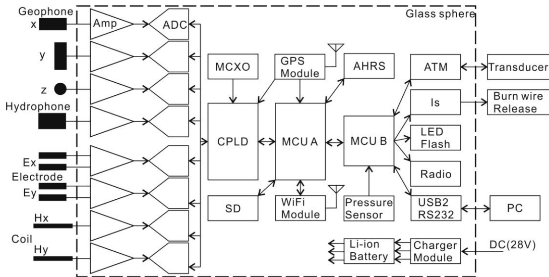
Fig. 3. Circuit diagram of the OBEMS data logger, containing EM and seismic sensors, eight amplifiers, eight analog to digital converters (ADC), a complex programmable logic device (CPLD), secure digital memory card (SD), microprocessor controlled crystal oscillator (MCXO), Li-ion rechargeable battery, charger module, LED Flash, Radio, ATM, and attitude heading reference system (AHRS). In this preliminary design, the ATM, burn wire release, ultra-short base line (USBL), and relay release are all designed for release.
