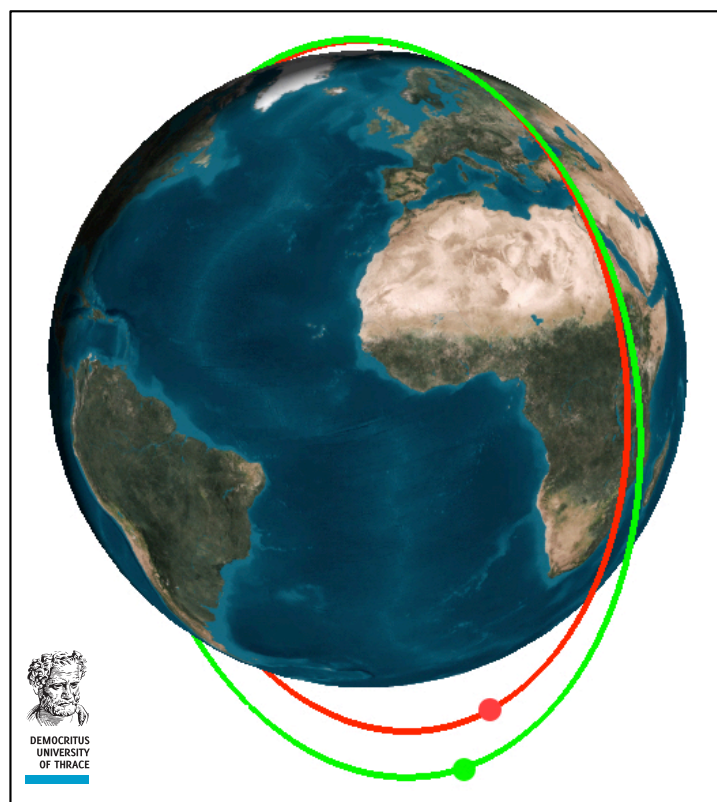
Figure 1: Simulated orbits of the main Daedalus satellite (green) and of a deployed sub-satellite (red).
