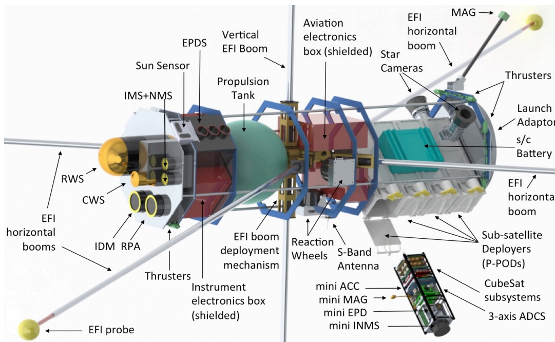
5 Figure 16: Interior of the main Daedalus satellite, including key s/c subsystems and instrumentation. A deployed CubeSat sub-satellite is also shown, with examples of potential sub-satellite miniaturized instrumentation.
