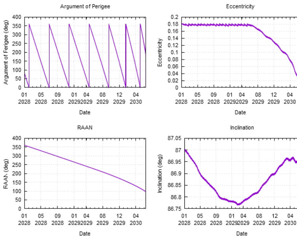
Figure 14: Long term evolution of Daedalus' Argument of Perigee, Inclination, Right Ascension of the Ascending Node and Eccentricity.
