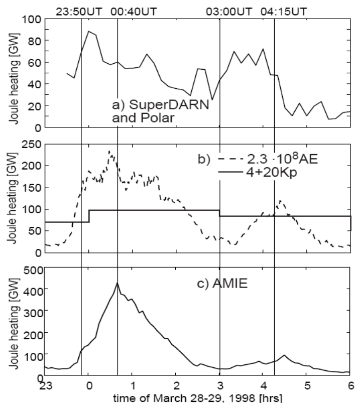
Figure 3: Discrepancies between global integrated Joule heating as estimated by (a) SuperDARN and Polar measurements, (b) AE- and Kp-based proxies, and (c) AMIE procedure during a solar storm (from Palmroth et al., 2005).
