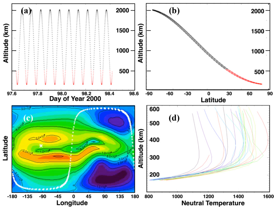
Figure 13: (a) Altitude vs. time for 10 Daedalus orbits; (b) altitude vs. latitude. Red dots: measurements below 500 km. (c) Horizontal sampling (d) vertical sampling of neutral temperature from NRLMSISE along 10 consecutive orbits, during the April 2000 storm.
