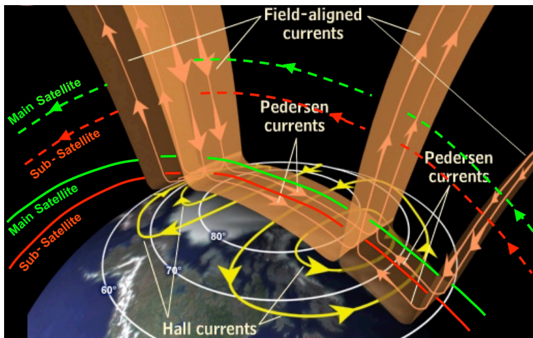
5 Figure 12: Measurement scheme by the main s/c (green) and a released sub-satellite (red), when apogee is at high latitudes (dashed lines) and when perigee is at high latitudes (solid lines). [adapted from: Gang Lu, The Comet Program, 2007]
