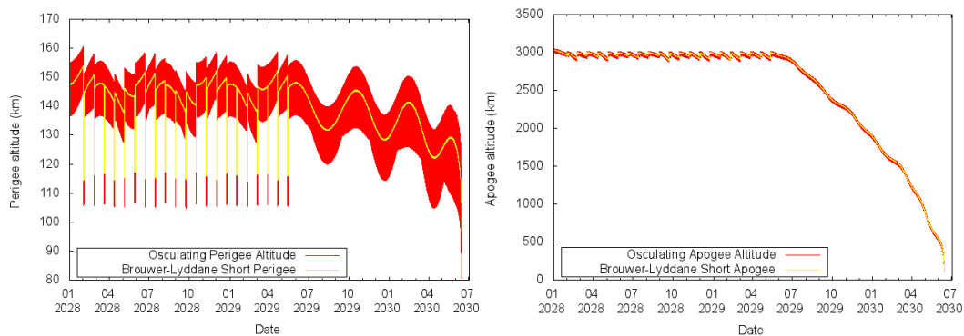
Figure 10: Daedalus perigee (left) and apogee (right) history for a spacecraft launch in 2028, initial apogee at 3000 km and initial satellite mass of 400 kg (including propellant). Apogee and perigee maintenance are employed by means of propulsion.
