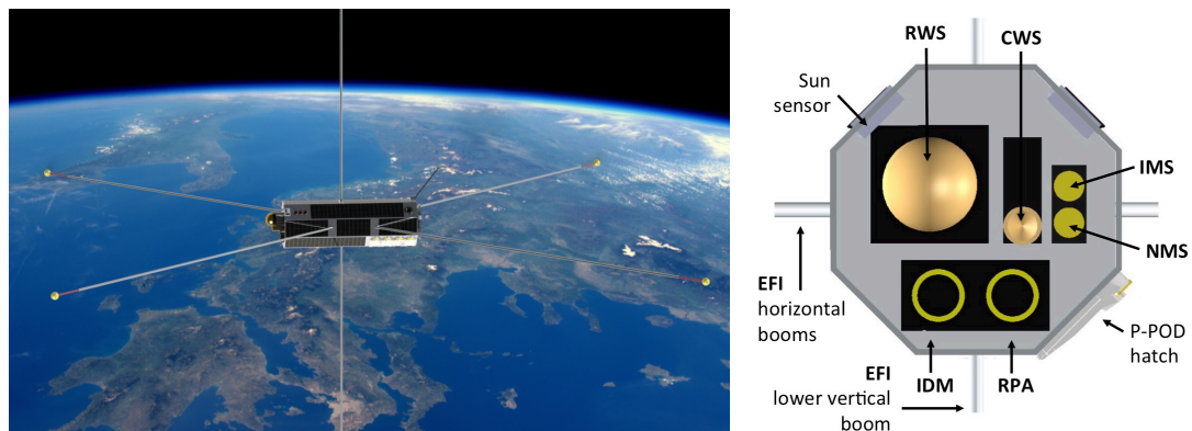
Figure 11: Spacecraft observation geometry: Daedalus s/c with extended field booms; four electric field booms are arranged in X-formation in the along-cross-track plane and two booms are aligned vertically (left). Ram direction instrumentation (right).
