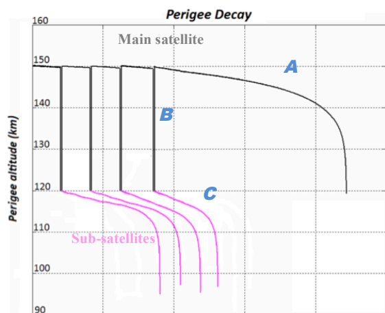
5 Figure 9: Schematic of the main phases of the perigee history for the Daedalus main satellite (gray lines) and four sub-satellites (magenta lines). The sub-satellites are released during four corresponding descents (“deep-dips”) of the main satellite down to 120 km.
