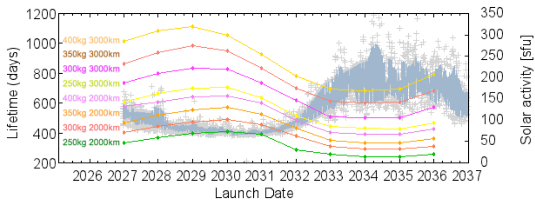
10 Figure 6: Simulated Daedalus lifetimes as a function of launch date, for a perigee of 150 km and for various values of apogee and spacecraft mass, as marked. It is noted that higher mass and apogee lead to longer lifetimes, whereas higher levels of solar activity lead to shorter lifetimes. Solar activity is plotted in terms of daily (grey crosses) and average (grey lines) values of the F10.7 index.
