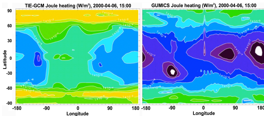
Figure 7: Joule heating from TIE-GCM (left) and GUMICS (right) for the storm of April 6th, 2000 (from Sarris et al., 2013)
