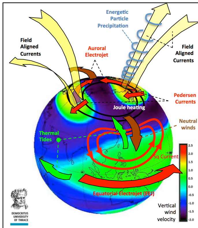
Figure 2: Overview of main processes affecting momentum and energy transport and distribution in the LTI.
