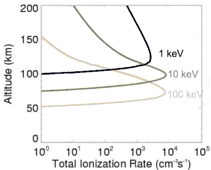
Figure 4: Total Ionization Rates vs. altitude at various energies of precipitating electrons, as marked.
