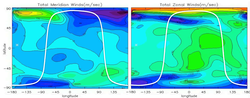
Figure 8: Simulations of Meridional and Zonal winds and ground track of a spacecraft orbit
