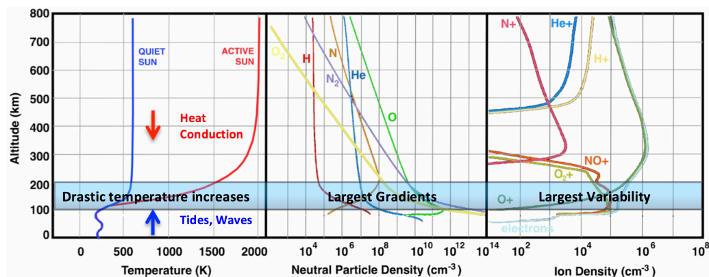
Figure 5: Simulated key variables in the LTI as a function of altitude: Temperature at quiet and active solar conditions (left), neutral (center) and ion (right) constituents. The altitude range from 100 to 200 km shows the largest rates of change in most variables.
