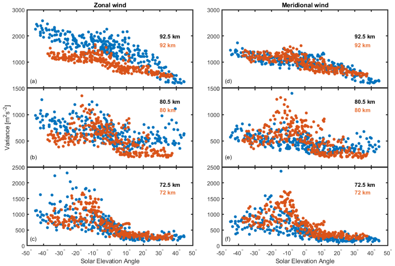
Figure 8. Zonal (left) and meridional (right) wind variance from the Rothera (blue) and Halley (Orange) radar for three altitudes, as a function of solar elevation angle.
