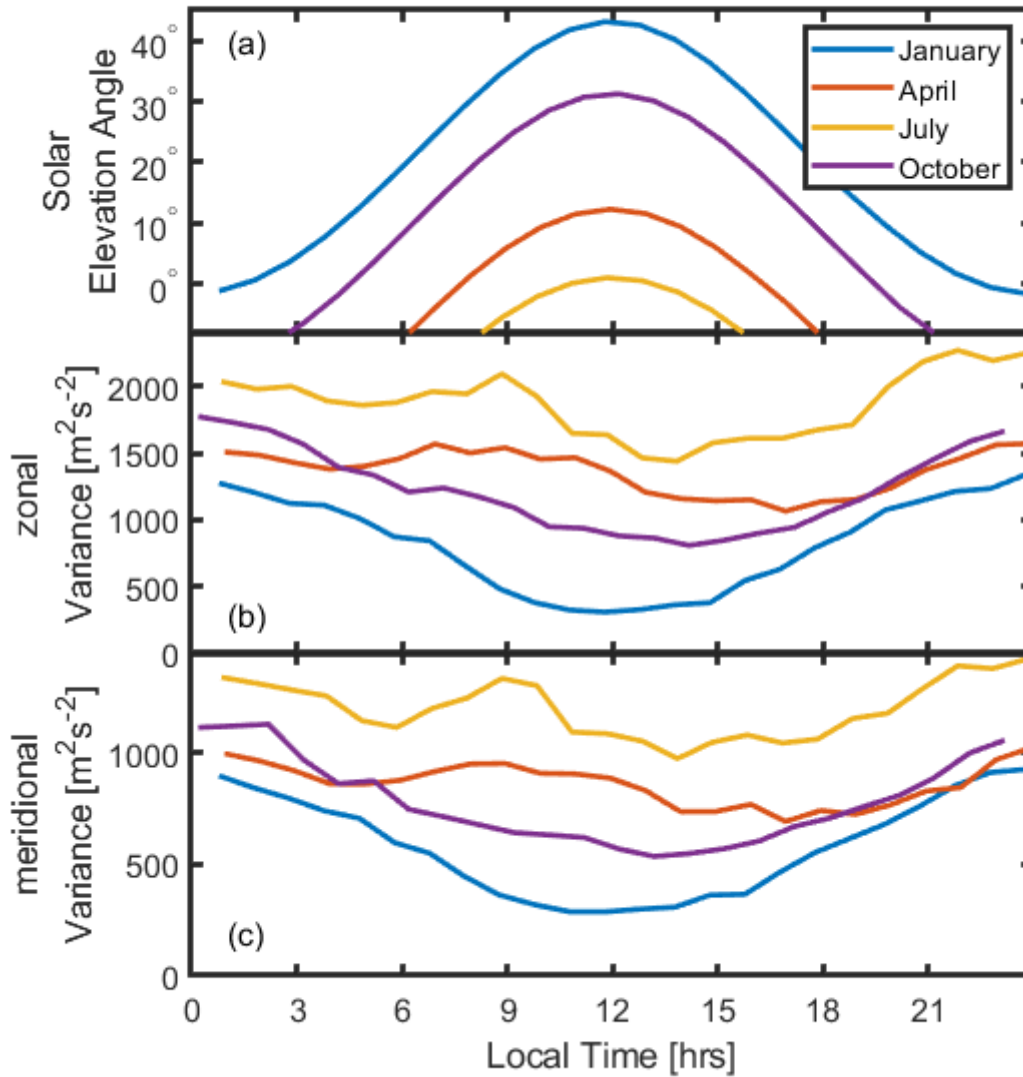
620 Figure7: (a) The average solar elevation angle for the 4 months indicated as a function of local time at Rothera, (b) the average daily cycle of zonal variance averaged over range gates from 88.5 to 90.5 km km for the same months: January (blue), April (red), July (yellow) and October (purple), (c) the same but for meridional variance.
