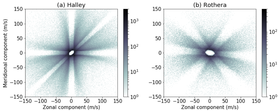
610 Figure 5. Two-dimensional density plots of wind velocity measurements with ellipse axial ratio R > 5 . Data points from all altitudes are included. The data from both radars show qualitatively similar patterns which seem to be artefacts of the 3-antenna arrangement and full-correlation analysis measurement technique.
