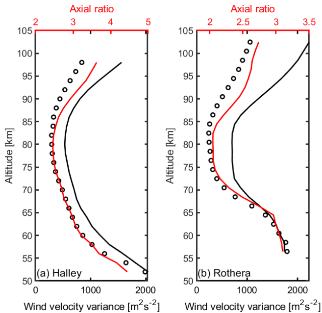
615 Figure 6. Vertical profiles of observed hourly variances in zonal wind data, excluding velocities over 150 \text{ ms}^{-1} (black), the expected hourly variance based on the observed number of outliers (black circles), the mean axial ratio (red).
