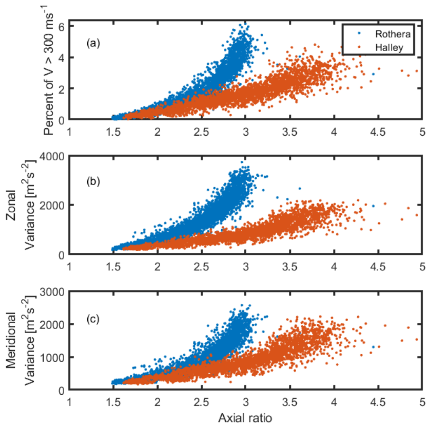
625 Figure 9. The relationship between axial ratio and (a) outliers and (b) hourly variance of the zonal wind and (c) hourly variance of the meridional wind. Each point represents a different hour, month and altitude, to isolate the effect of differing error levels. Only altitudes over 80 km are shown. Meridional and zonal winds show substantially the same relationship, with slightly smaller variances in the meridional direction (reflective of the lower wind values).
