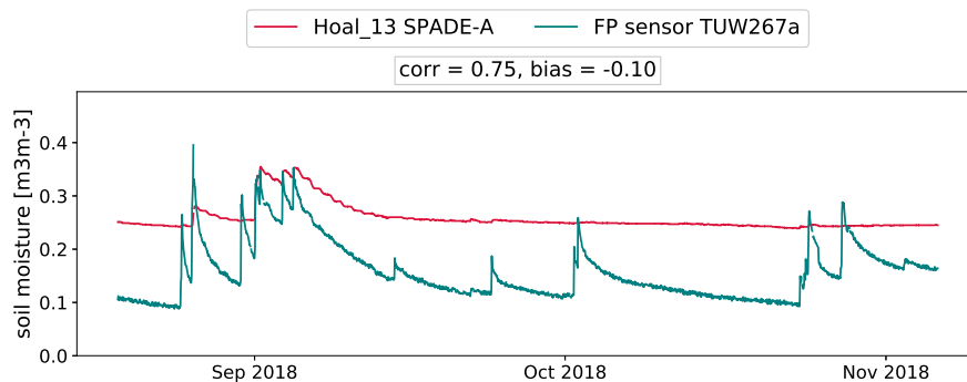
Figure A2. Soil moisture time series of FP sensor TUW267a and professional probe Hoal_13 at 0.05 m depth, installed next to each other. While the low-cost sensor shows distinct peaks due to rain events, the professional probe reacts considerably weaker.
