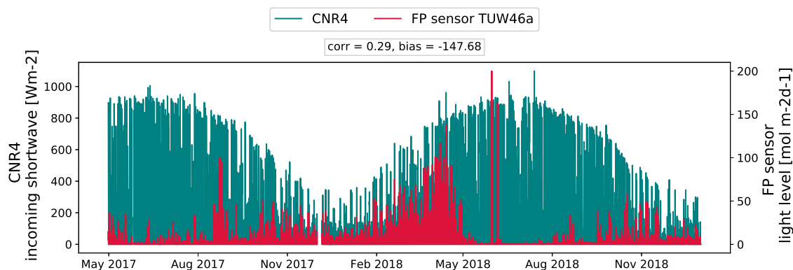
Figure 7. Same as Fig. 6, but for FP sensor TUW46a (located in sparse forest).
