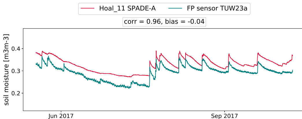
Figure 9. Soil moisture time series of FP sensor TUW23a and professional probe Hoal_11 at 0.05 m depth, installed next to each other, in good agreement.
