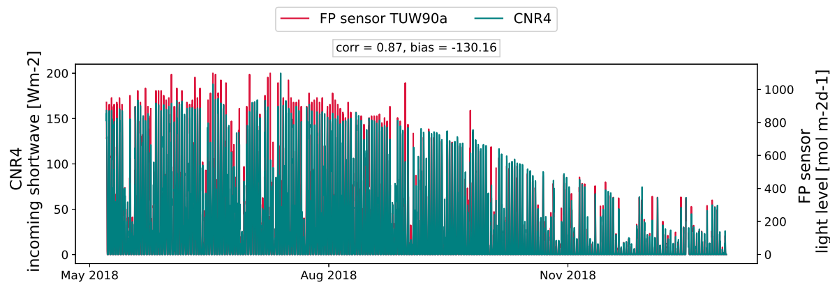
Figure 6. Light level variable observed with the FP sensor TUW90a expressed in \text{mol m}^{-2}\text{d}^{-1} plotted against the incoming shortwave radiation in \text{Wm}^{-2} from the professional probe CNR4.
