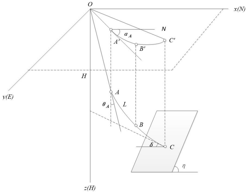
Fig. 1. Coordinate system of borehole trajectory
