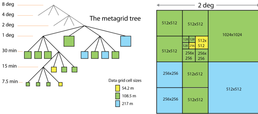
205 Figure 2. (left) An example of a quadtree metagrid tree structure with a 2 deg subsection color coded to illustrate different data grid resolutions in meters. (Note that a 960 x 960 grid subtending 1 degree has-would have a grid cells size of 115.7m). (right) The same subsection is shown as a map. Numbers in the square areas illustrate grid sizes used to achieve different spatial resolutions.
