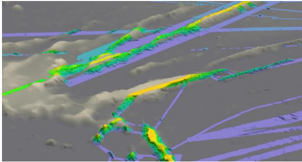
Figure 8. In this example, a low resolution grid has been used to fill in around a high resolution multibeam data. Two colormaps are used with a highly saturated colors being used to highlight multibeam data.
