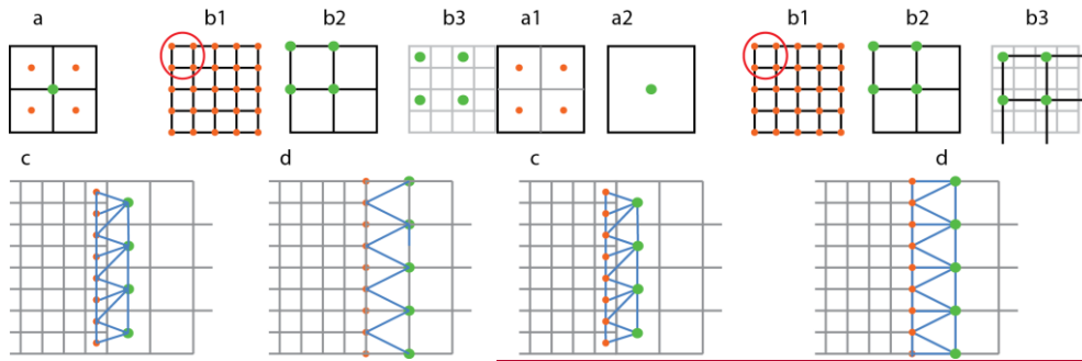
Figure 1a) when depths values placed at the centers of cells are averaged to a lower resolution, the result is also at the center of a cell (a2). b) the averages of four point-vertex groups do not lie on vertices (b2) but at the centers of grid cells (b3) so there are no common vertices between grids at different scales. c) and d). Triangle strips linking adjacent grids are topologically the same for the two schemes.
