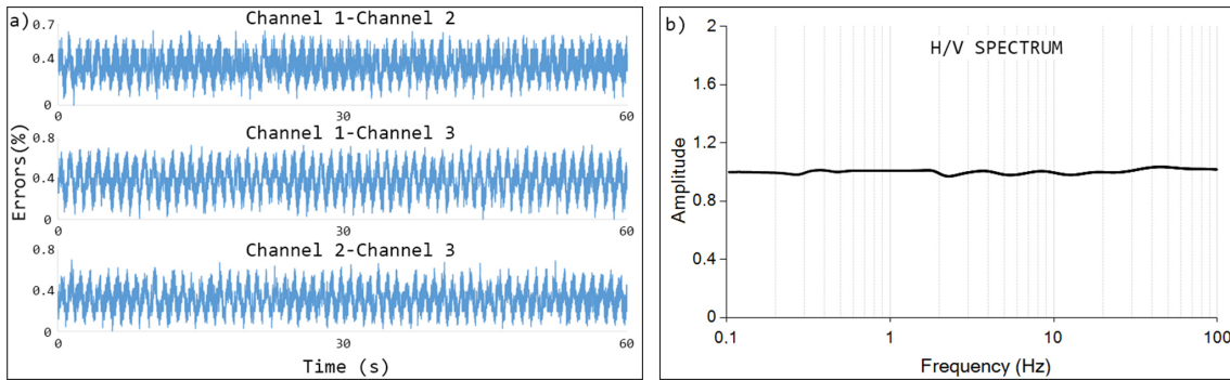
Figure 4. a) Error percentage of difference signal estimated during the first channel consistency test b) H/V spectral ratio.
