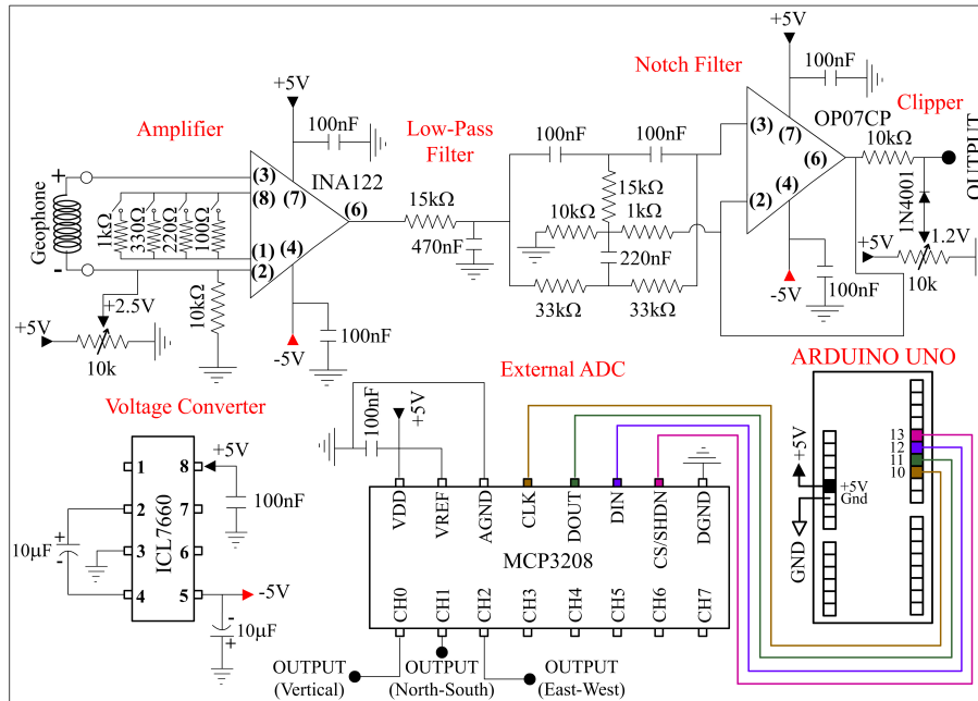
Figure 3. Schematics of external hardware and pin connections.
