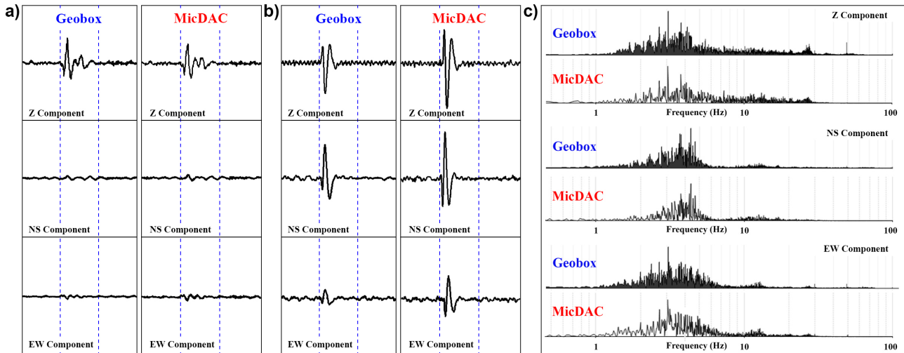
Figure 8. Three-component seismic data recorded simultaneously using both devices a) MicDAC with 46 dB gain b) MicDAC with 60 dB gain c) Comparison of Fourier spectra of recorded three-component microtremor data using GeoBox and MicDAC.
