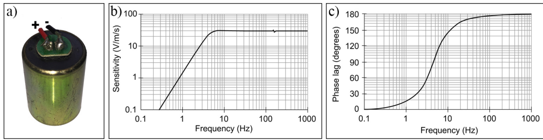
Figure 2. For the geophones with 4.5 Hz natural frequency a) External view b) Amplitude response c) Phase response.
