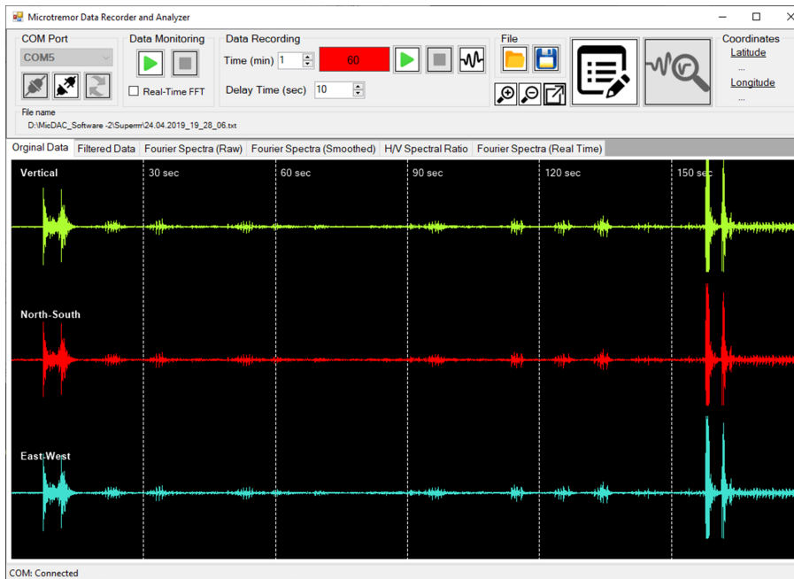
Figure 5. Screenshot of MicDAC-GUI and detected signals using a 4.5 Hz vertical geophone connected to each channel inputs.
