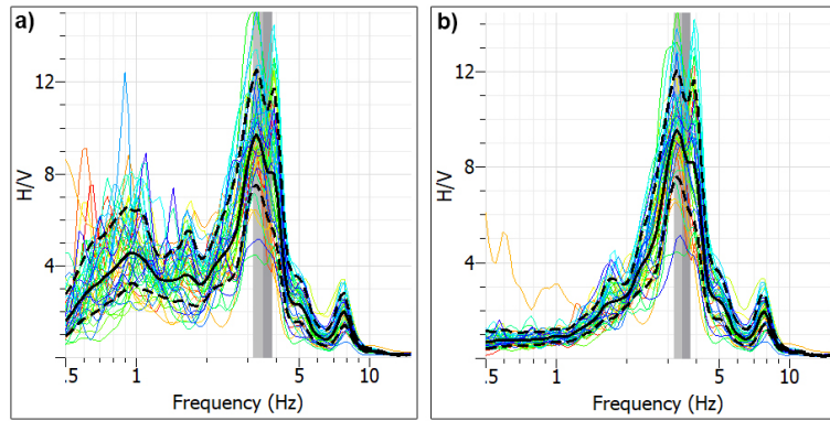
Figure 9. The obtained H/V spectral ratios of recorded data by a) GeoBox b) MicDAC.
