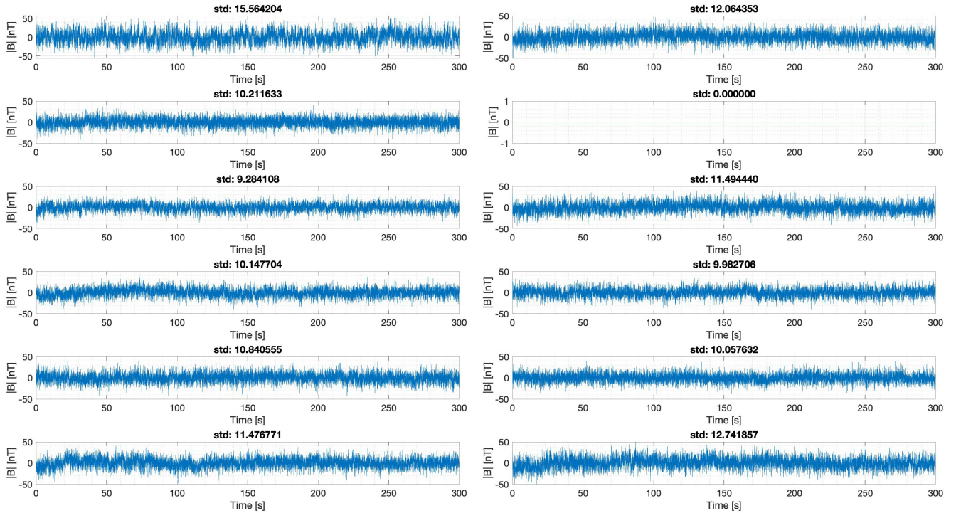
Figure 10. Pre- and post-exposure (left and right panels respectively) measurements of the magnetic field inside the Zero-Gauss chamber at the University of Michigan for the six sensors used during the GSFC test campaign.
