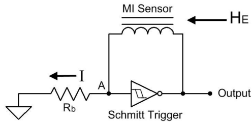
Figure 1. Basic circuit showing the working principle of the magneto-inductive technology. The Schmitt trigger flips the direction of the current that causes the sensor to charge and discharge in both directions (from Leuzinger and Taylor 2010).
