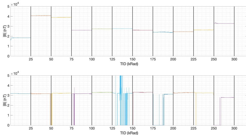
Figure 7. Magnitude of the magnetic field as measured by sensors 4 (top) and 5 (bottom) during the test campaign at the GSFC. The data shown between vertical lines correspond to two-minutes intervals collected between exposures. The vertical lines mark the TID that the sensors went through before taking the measurements.
