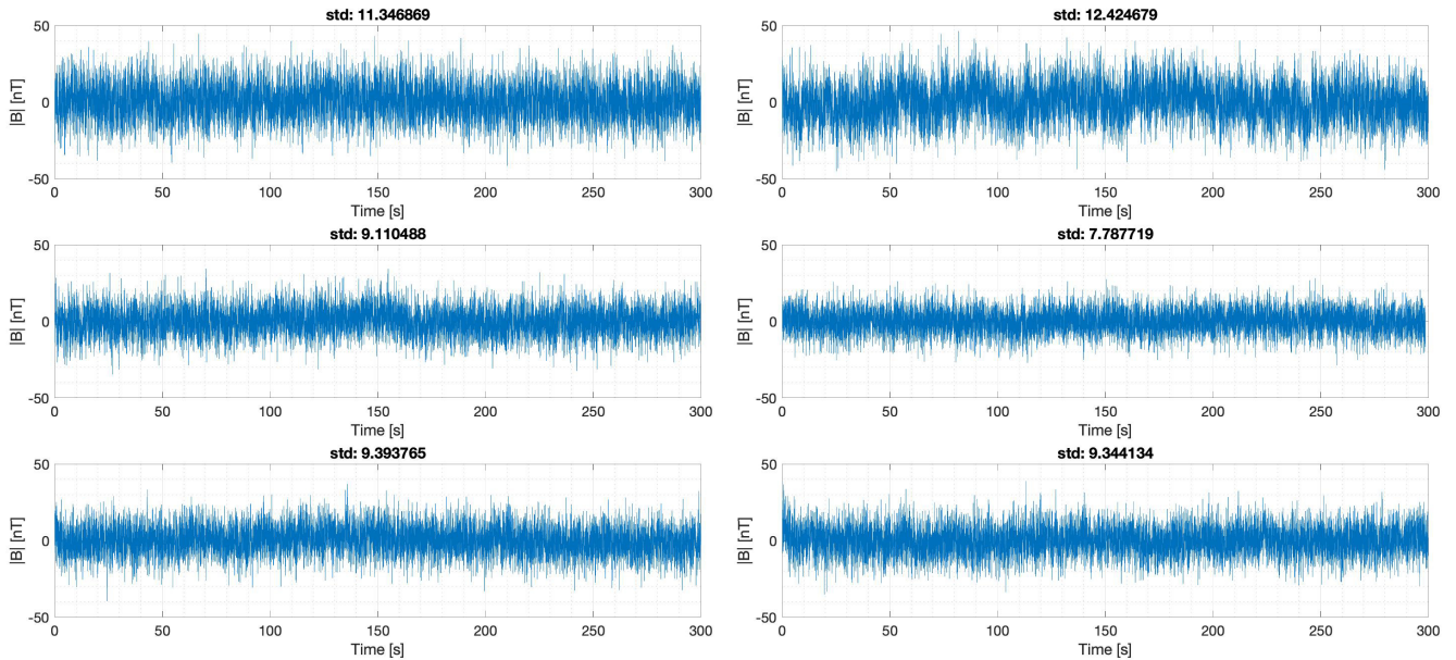
Figure 9. Pre- and post-exposure (left and right panels respectively) measurements of the magnetic field inside the Zero-Gauss chamber at the University of Michigan for the three sensors used during the University of Michigan test campaign.
