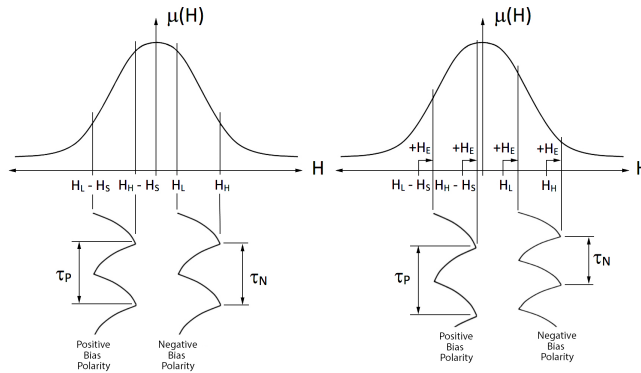
Figure 2. Permeability curve of the core material of the sensors, showing region of operation and difference in charge and discharge times in the absence (left) and presence (right) of an external magnetic field (from Leuzinger and Taylor 2010).
