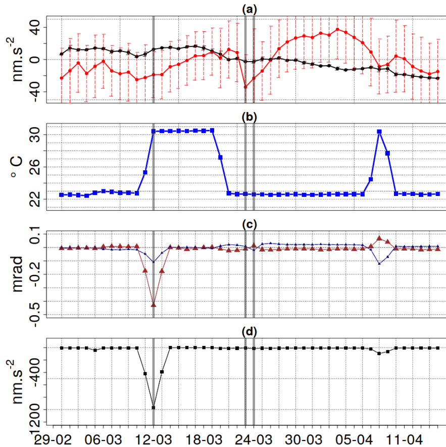
Figure 6. (a): Residuals of g for the iGrav-002 (black) and AQG-B01 (red). (b): external temperature (blue). (c): Tilts in x (brown) and y (dark blue) for the tests 3 and 4 in March and April 2020 (see Figure 1 for the timeline). (d): Tilt correction combined for x and y in \text{nm}\cdot\text{s}^{-2} . Dates marked as grey were subject to further instrument tests and adjustments.
