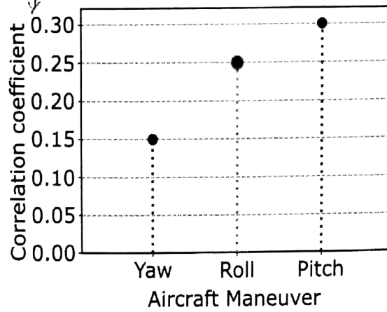
Figure 15. Correlation coefficient of the RMI and aircraft maneuvers.
