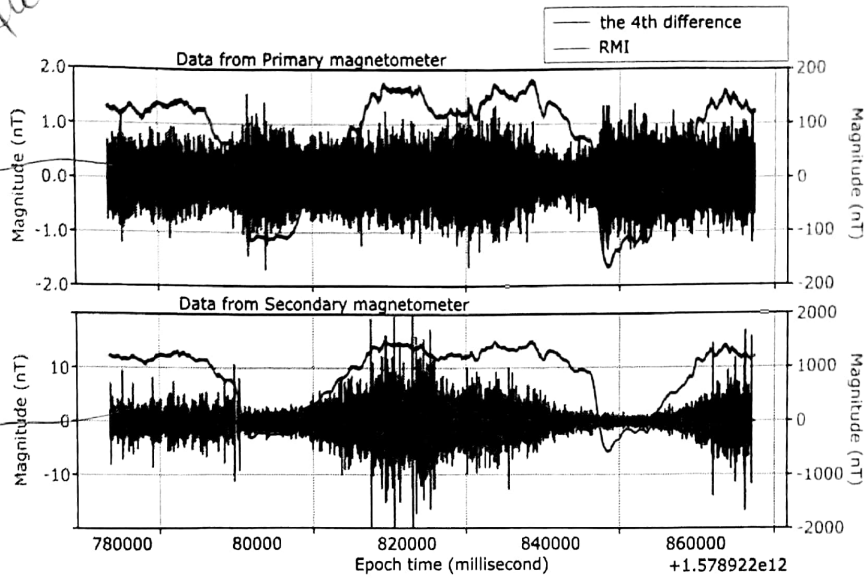
Figure 8. Data excerpt of the RMI by the primary and secondary magnetometer while the UAV was flown manually in the multi-rotor mode on 2020.01.13 with d = 20 cm and L = 20 cm. The IGRF (50560 nT) has been removed, constant removed?
