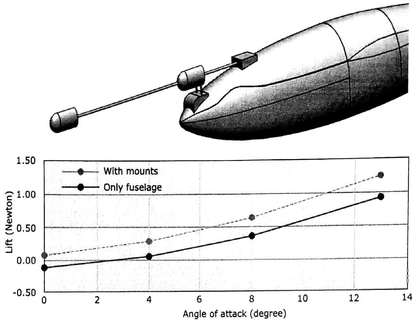
Figure 4. The nose-mounting solution and its aerodynamics simulation.
