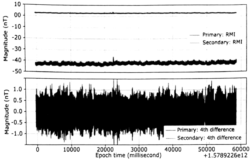
Figure 7. Data excerpt of the RMI and the fourth difference by the primary and secondary magnetometer while the UAV was on standby on 2020.01.13 with d = 20 cm and L = 20 cm. The IGRF (50560 nT) has been removed.
