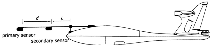
Figure 5. The final design of the front-boom-mounting setup and a side view of the hybrid VTOL fixed-wing in this study.
