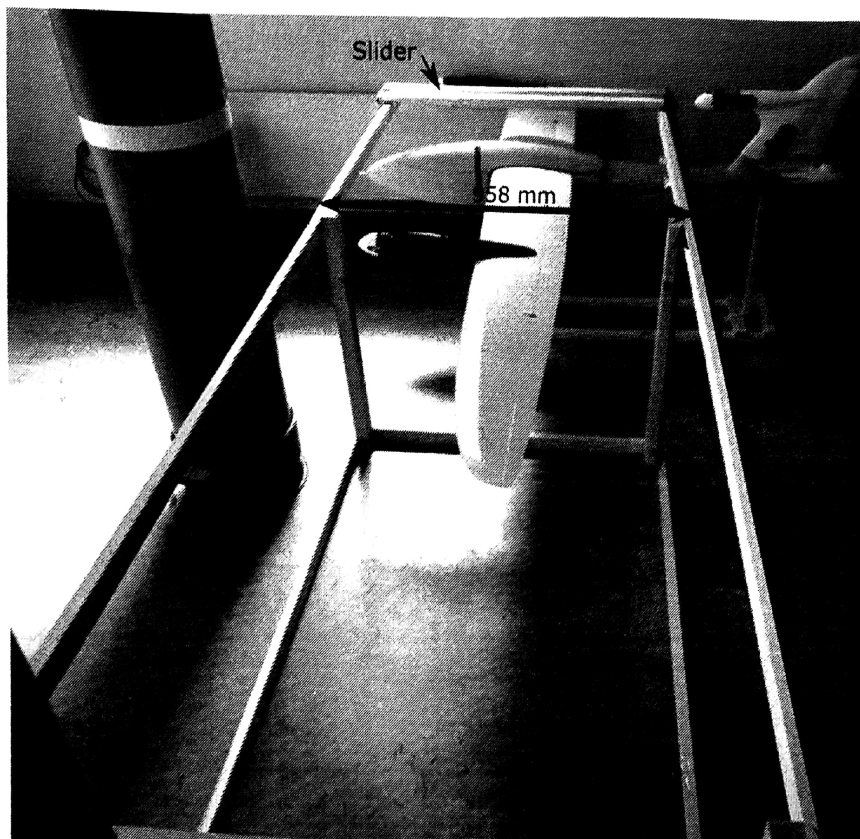
Figure 1. Demonstration of the magnetic signature measurement of the port wing. The length and width of the slider are 1000 and 150 mm, respectively.
