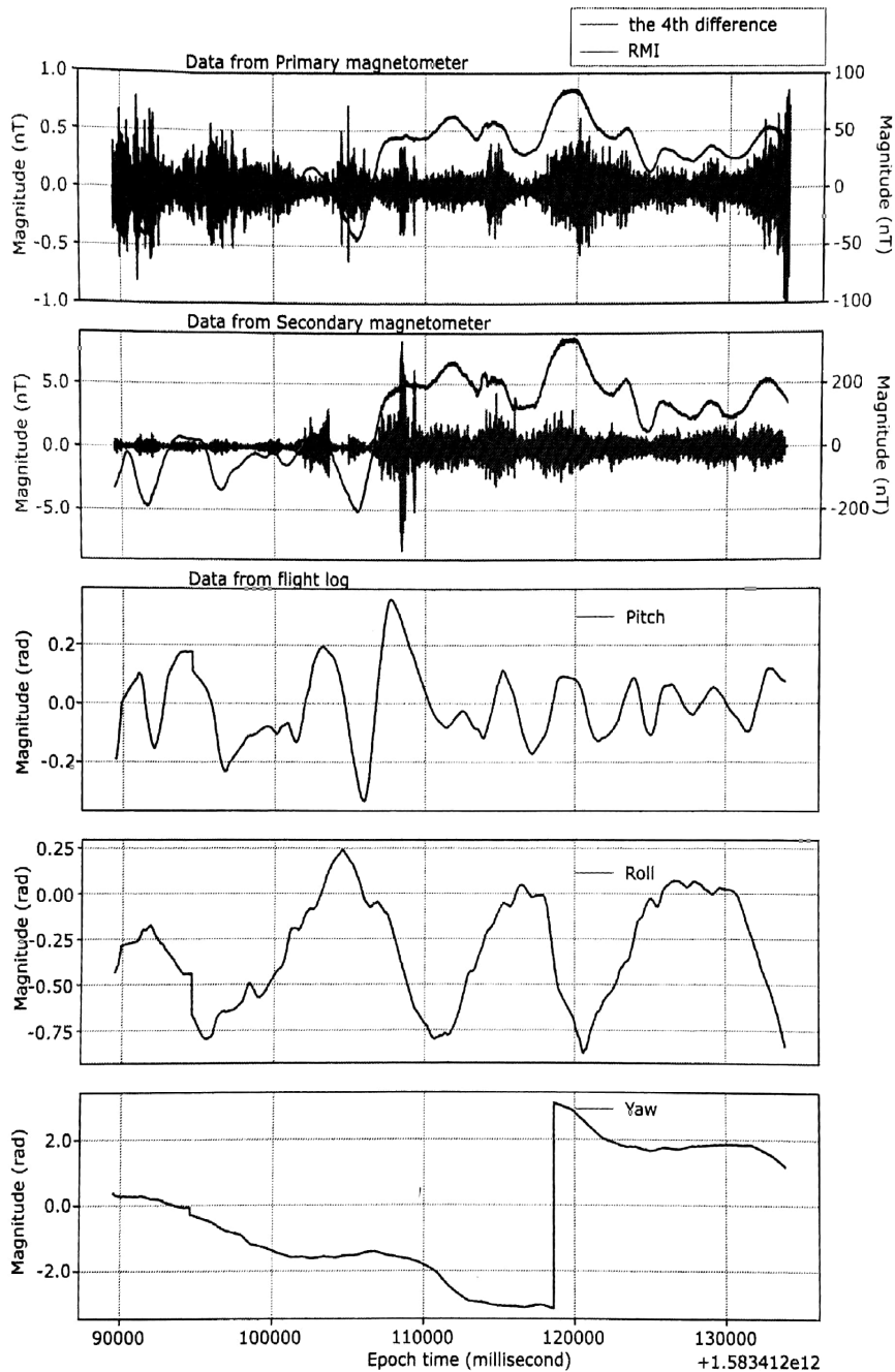
Figure 14. The RMI of the second segment from left to right in Fig 11 and 12 and the corresponding attitude from flight log.
