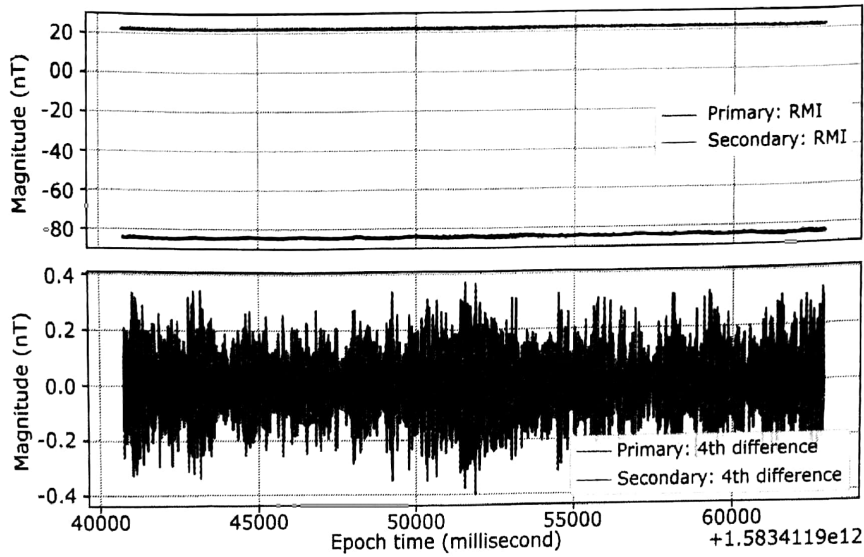
Figure 10. Data excerpt of the RMI and the fourth difference by the primary and secondary magnetometer while the UAV was on standby on 2020.03.05 with d = 20 cm and L = 30 cm. The IGRF (50563 nT) has been removed.
