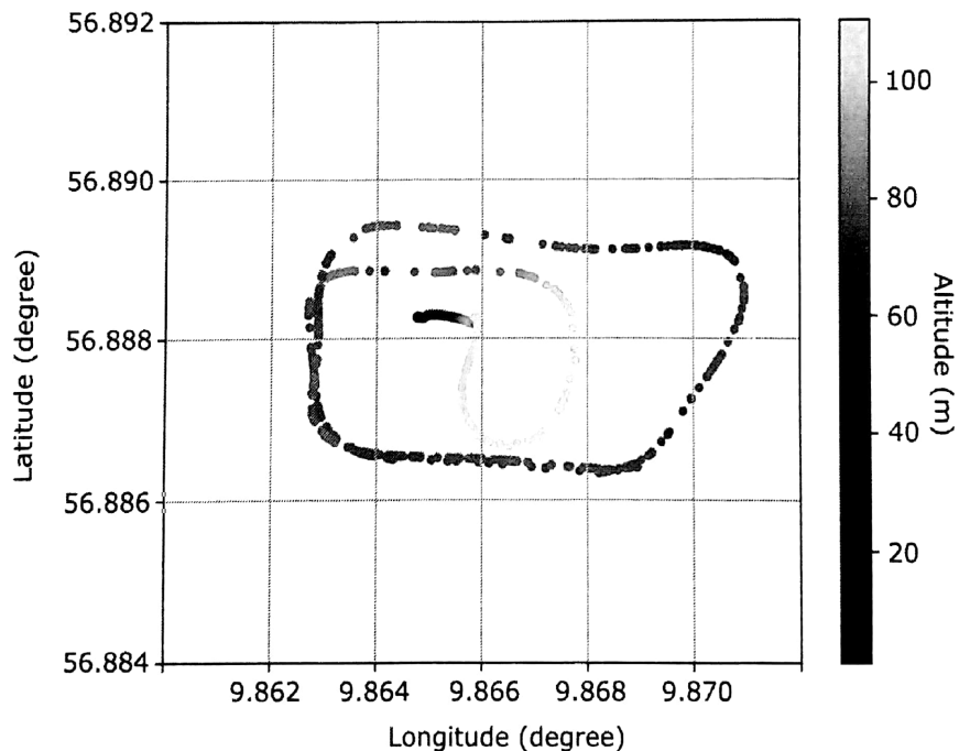
Figure 13. The production flight of the data excerpt. The altitude indicates the in-flight height above mean sea level.
