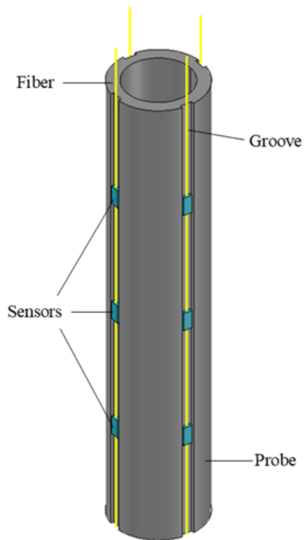
Figure 1: OFDR sensors installation method
