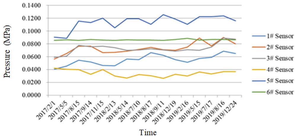
Figure 2: Monitoring data curves of multiple sensors
