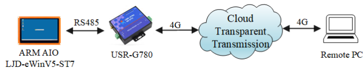
Figure 7: Connection topology.
