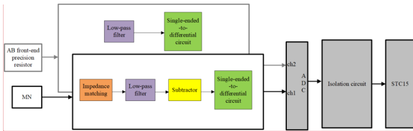
Figure 4: Block diagram of the AB.
