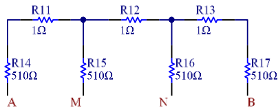
340 Figure 8: Schematic of resistor string connections for laboratory experiment.
