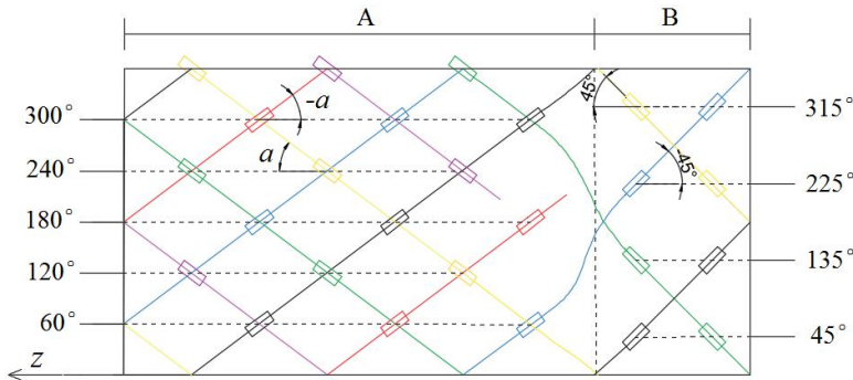
120 Figure 5: The layout position of the sensor group.
