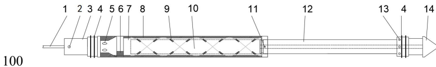
1 Sensing optical fiber 2 Locating pin 3 Mounting rod 4 block circle 5 threading hole 6 conductor groove 7 tube body 8 epoxy resin 9 FBG sensor group 10 Glue capsule 11 pin hole 12 piston rod 13 rubber outlet hole 14 conical guider
