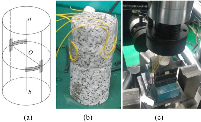
240 Figure 9: The layout diagram and photos of strain gauge.
