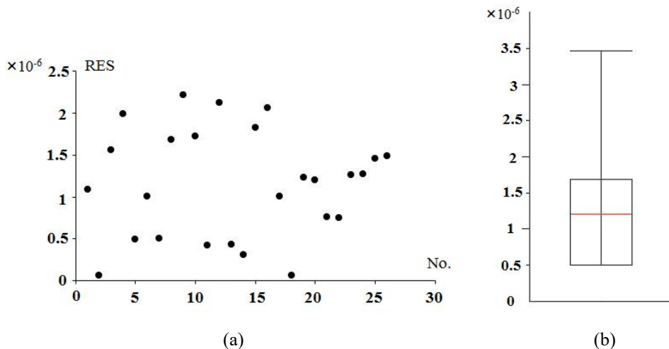
Figure 21: Residual error analysis of FBG strain measured data.
