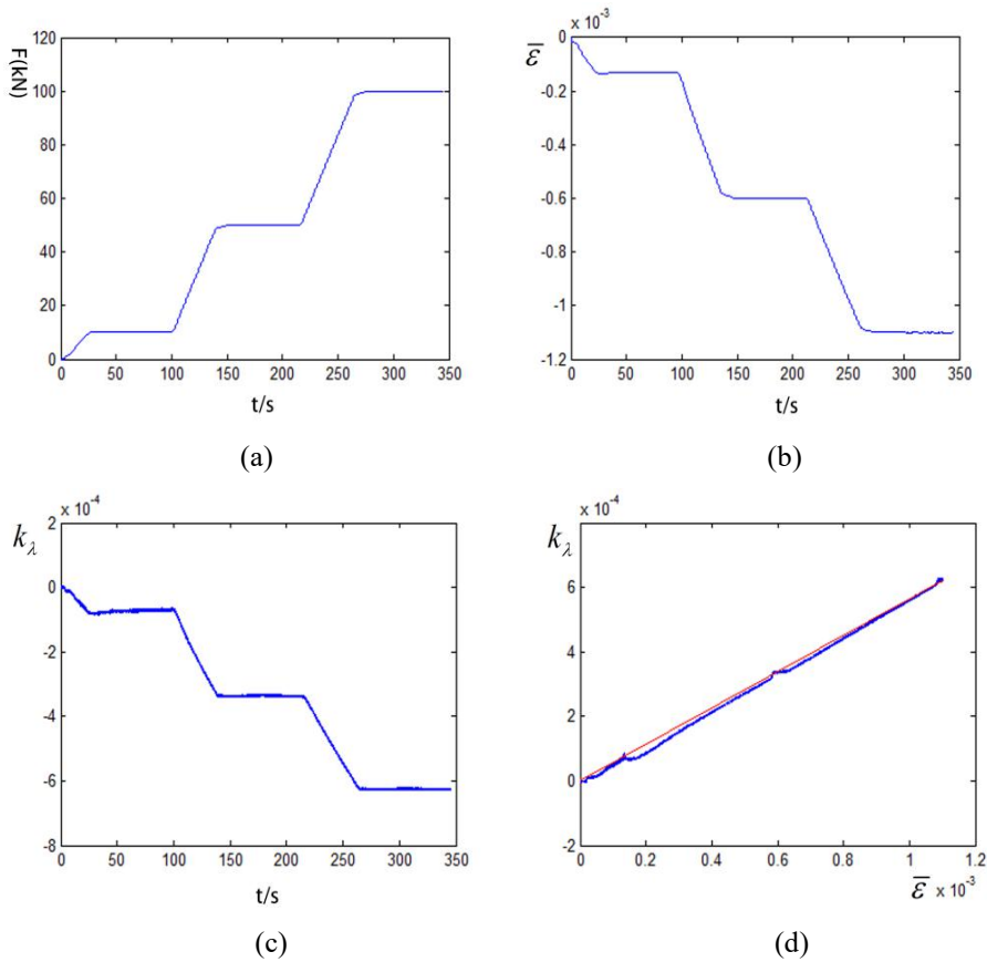
285 Figure 13: Schematic diagram of data processing in stress loading process.
