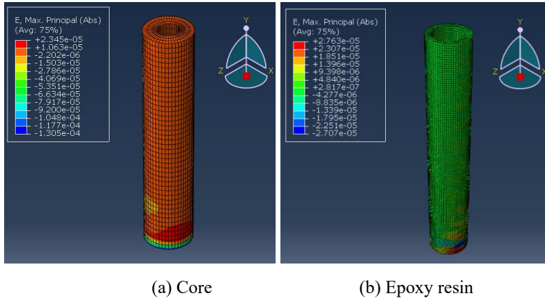
360 Figure 19: The absolute maximum principal strain nephogram of the core and epoxy resin after overcoring.
