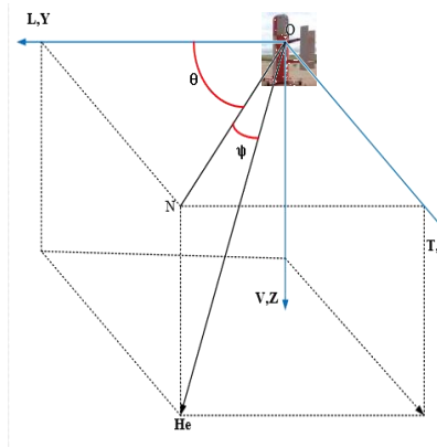
75 Figure 5: The towed bird coordinate system
